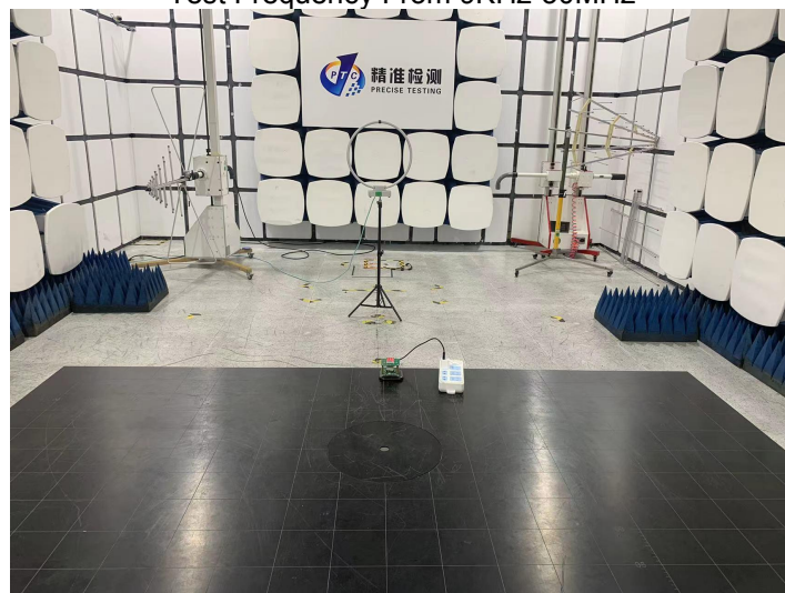
Radiated Spurious Emissions Test Frequency From 9KHz-30MHz
