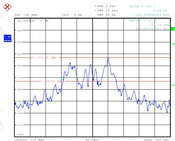
20dB Occupy Bandwidth 315MHz
