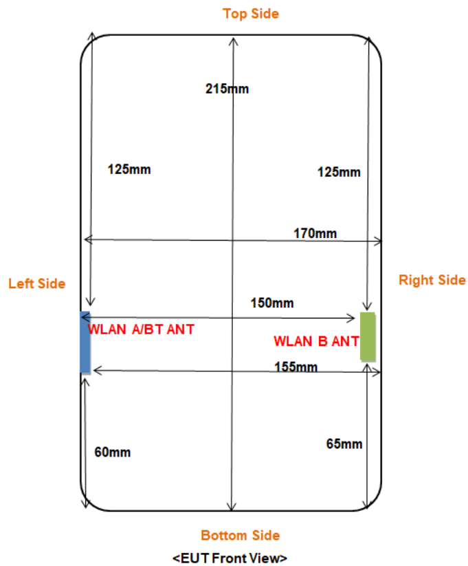
Fig 7.2 Block Diagram for EUT Antenna Position
