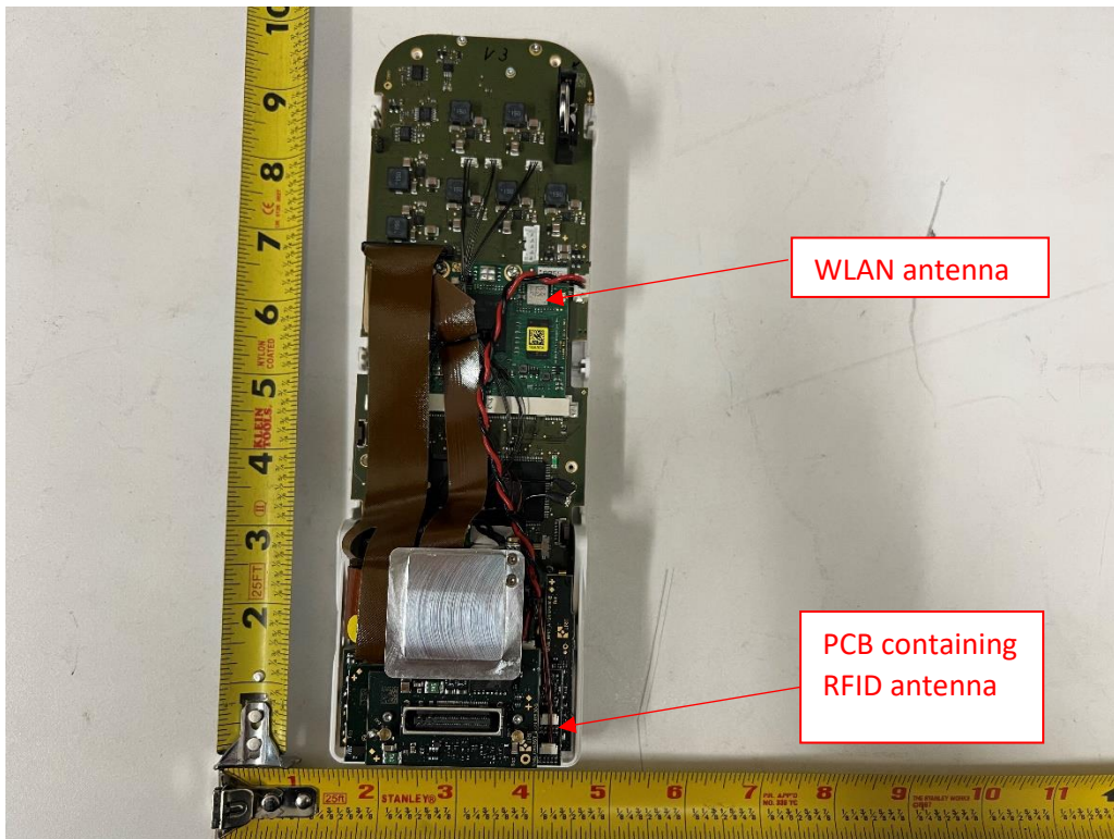
OPEN ENCLOSURE VIEW 2
