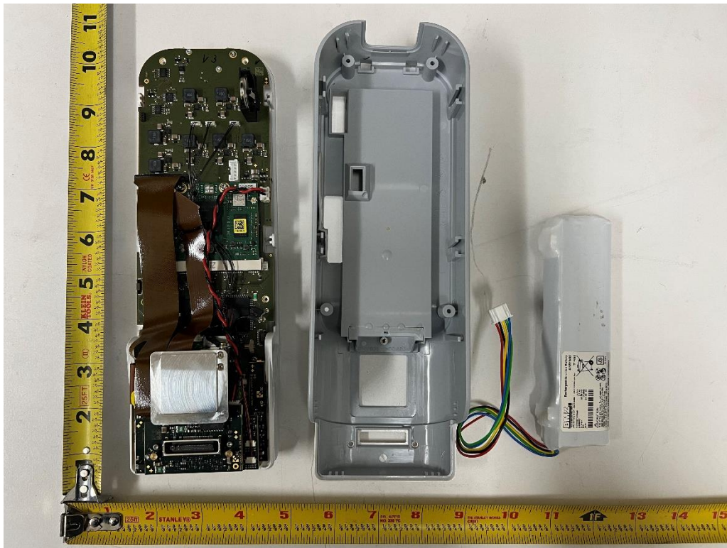
OPEN ENCLOSURE VIEW 1
