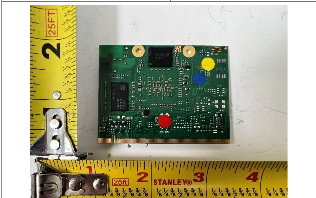
Sub-PCBA1 Bottom View
