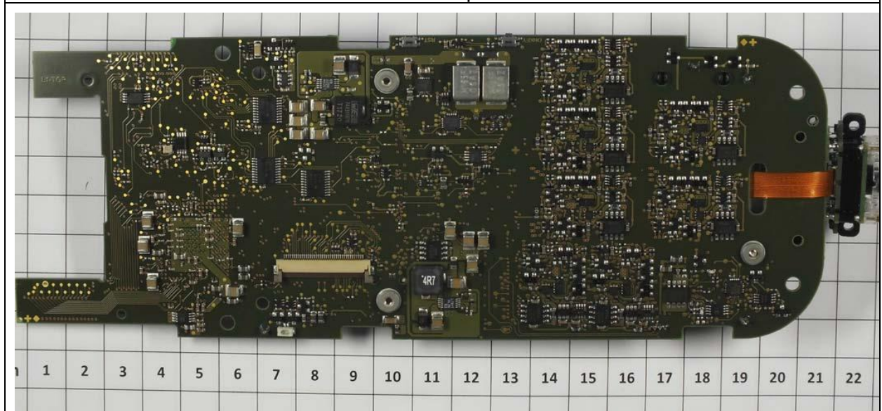
Main PCB Bottom View
