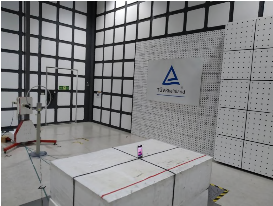
Photograph 3: Set-up for Radiated Emissions
