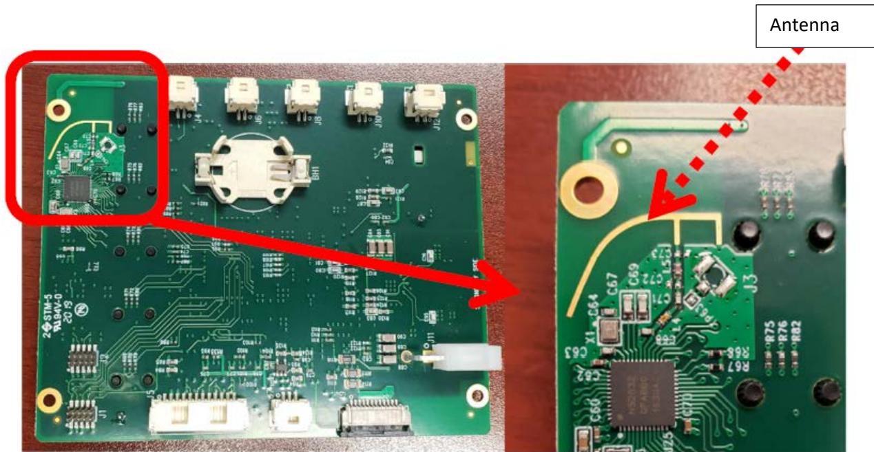
The antenna is a printed inverted F antenna, whose gain is about 1 dBi.
