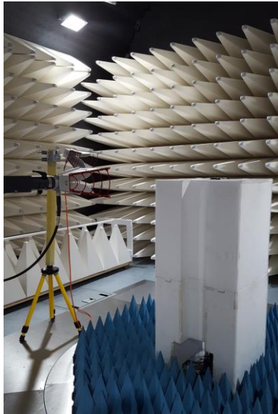
Figure C3. Radiated spurious measurement co-location setup High range
