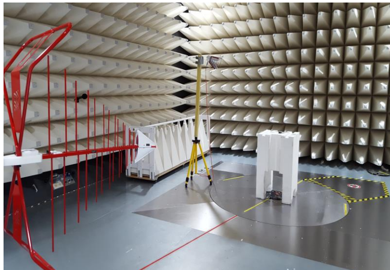
Figure C4. Radiated spurious measurement Co-location setup Low Range
