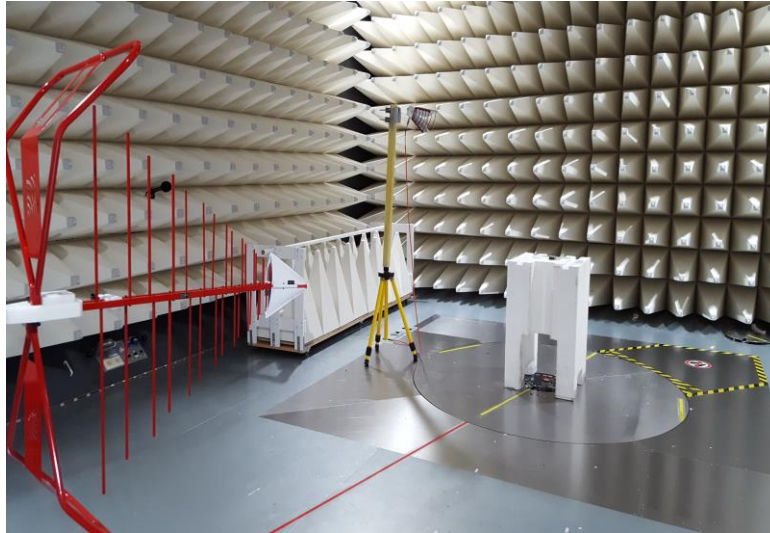
Figure B3. Radiated measurement setup Low range
