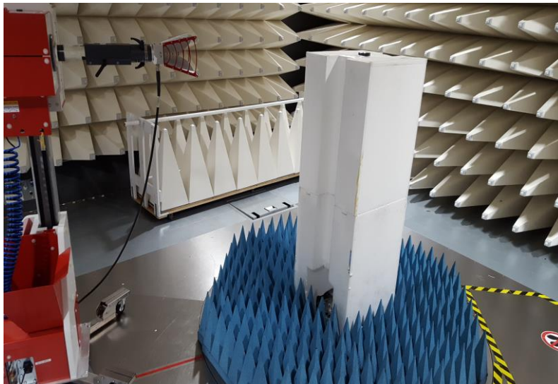
Figure B4. Radiated measurement setup High Range
