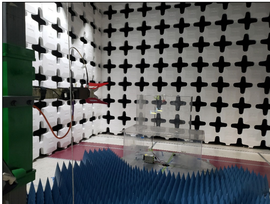
Photograph 2: Radiated Spurious Emissions, Above 1GHz, Test Setup
