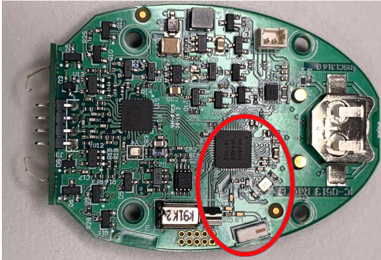
Antenna: RF ANT 2.4GHZ CHIP SOLDER SMD Radio: Nordic NRF52832-QFAA-R
