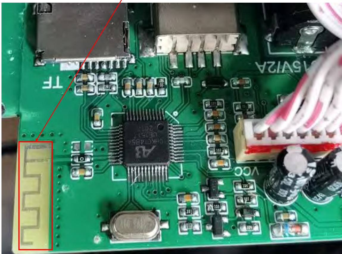
BT Antenna
