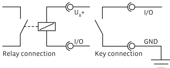
I/O connection (Top view)
