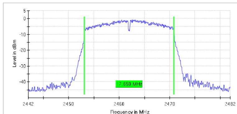
6 dB Bandwidth
