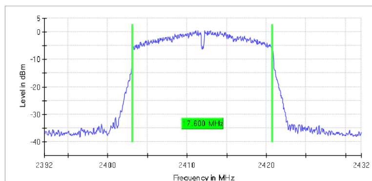
6 dB Bandwidth
