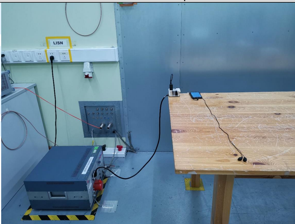
Conducted Emission Test Setup-3 - Mode 3
