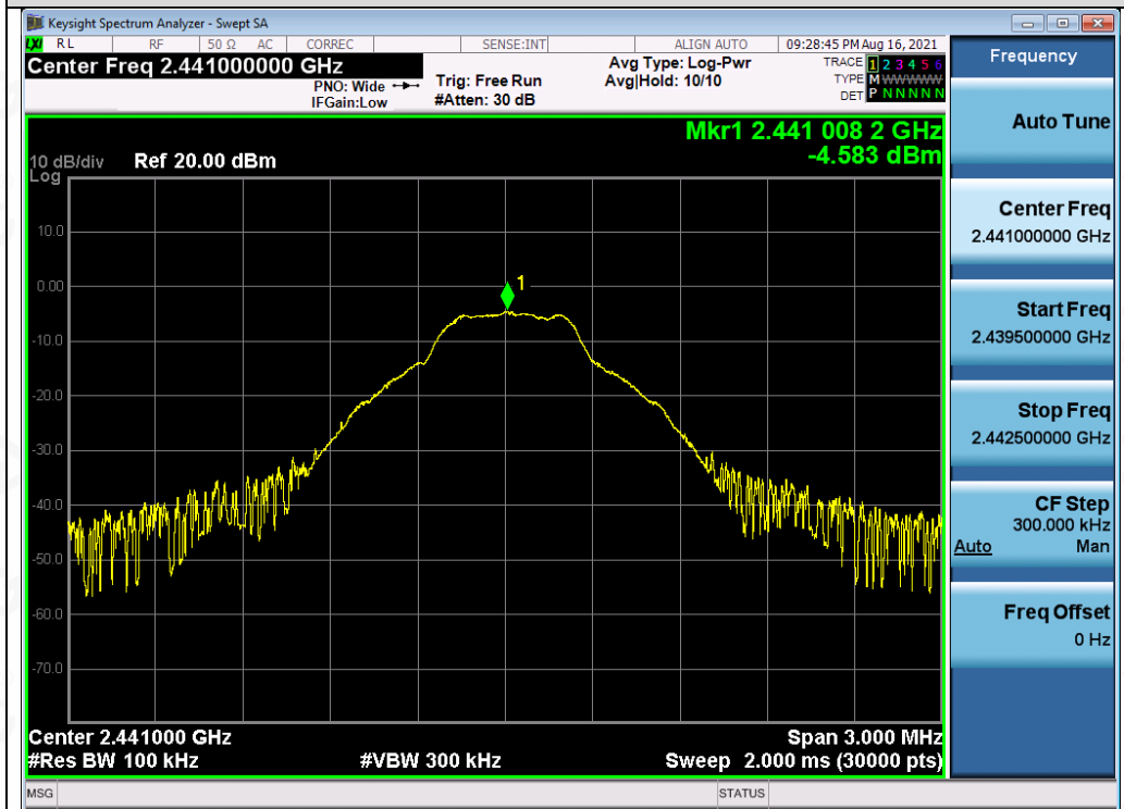
Test_Graph_BR_ANT1_2441_1Mbps_Reference Level
