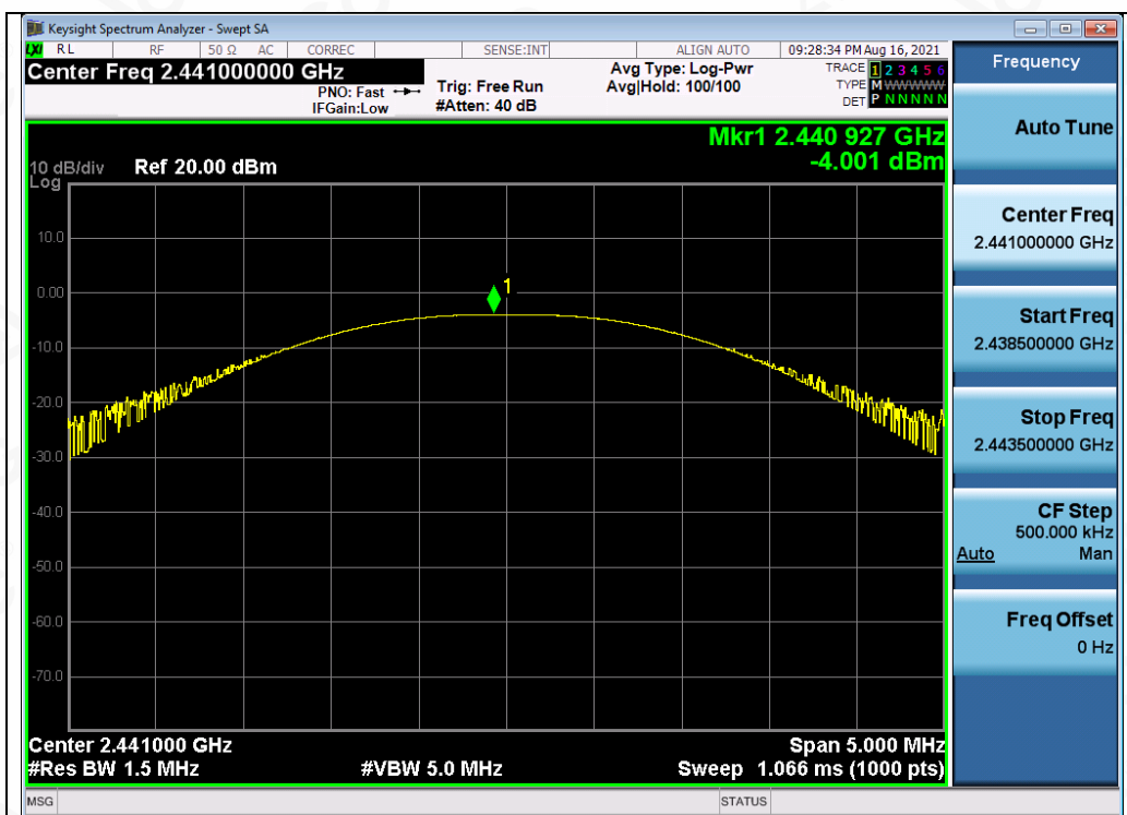
Test_Graph_BR_ANT1_2441_1Mbps_Peak Power
