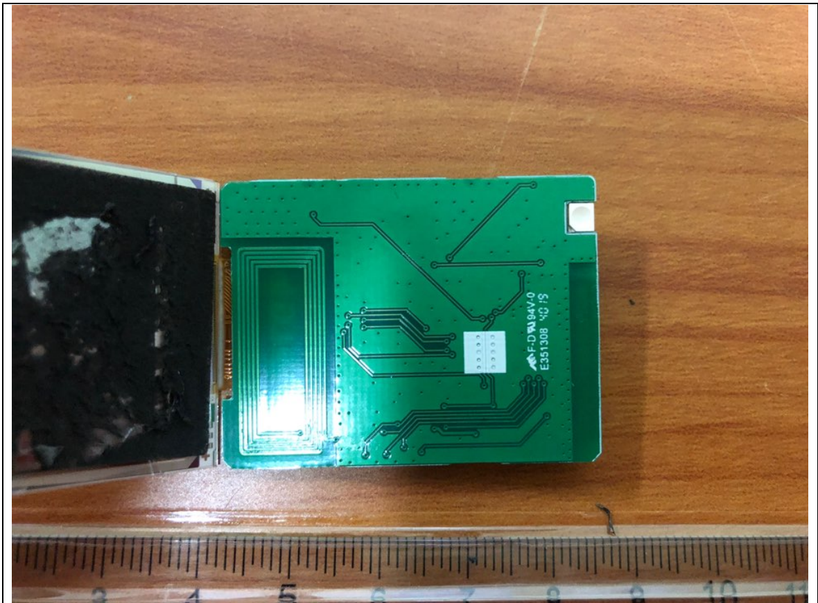
MainBoard-Rear
