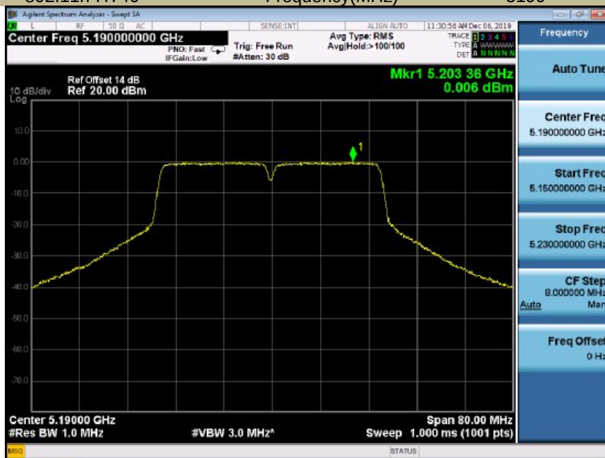
Power Spectral Density Test Model 802.11n-HT40
