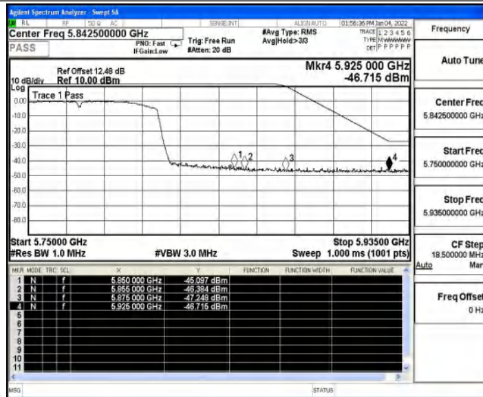
11AC80SISO_Ant0_High_5775_Peak
