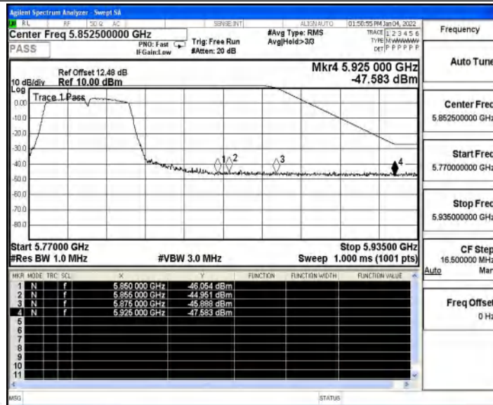
11AC80SISO_Ant0_Low_5775_Peak
