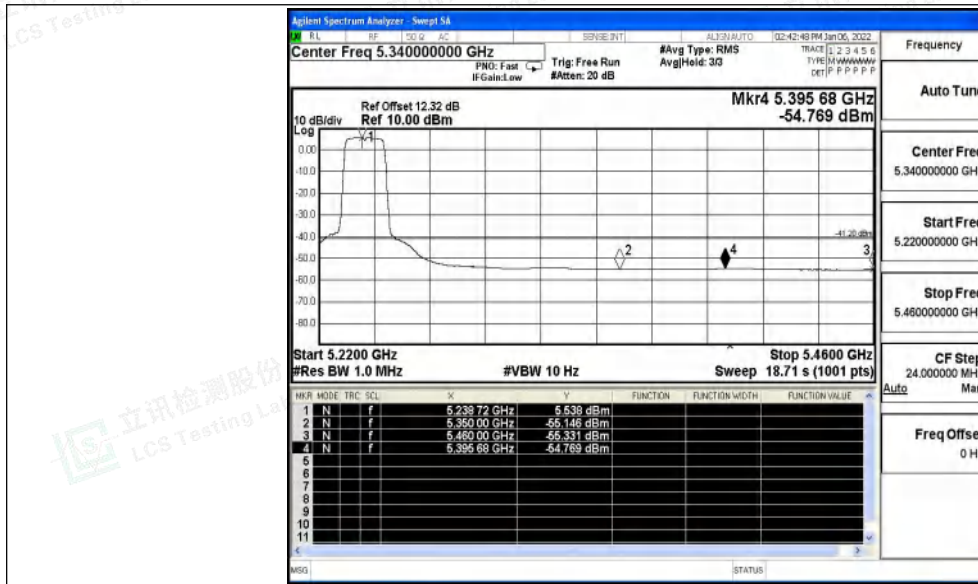
11A_Ant1_High_5240_Peak
