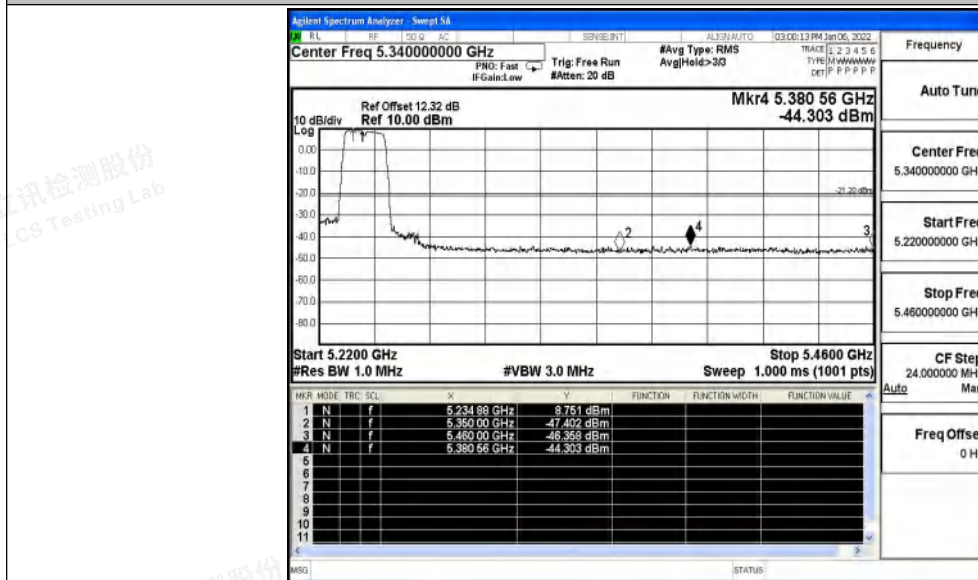
11N40SISO_Ant1_Low_5190_AV
