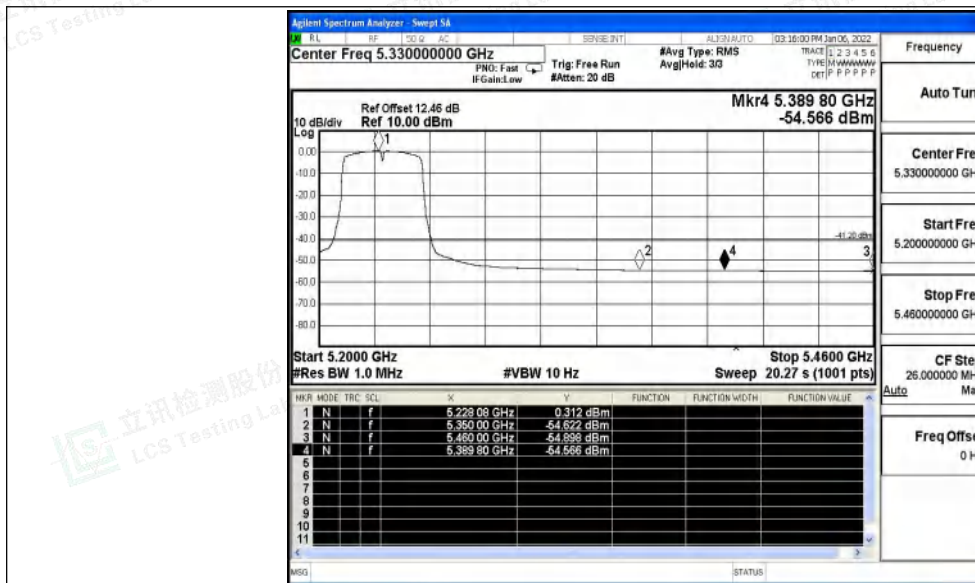
11N40SISO_Ant1_High_5230_Peak
