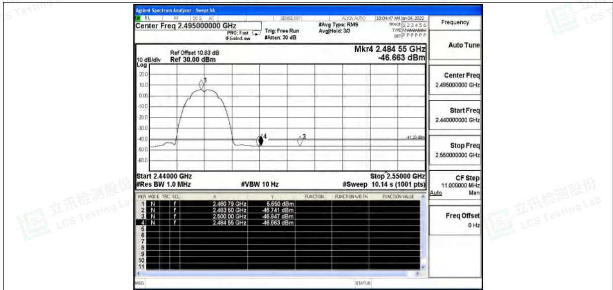
11B_Ant0_High_2462_Peak
