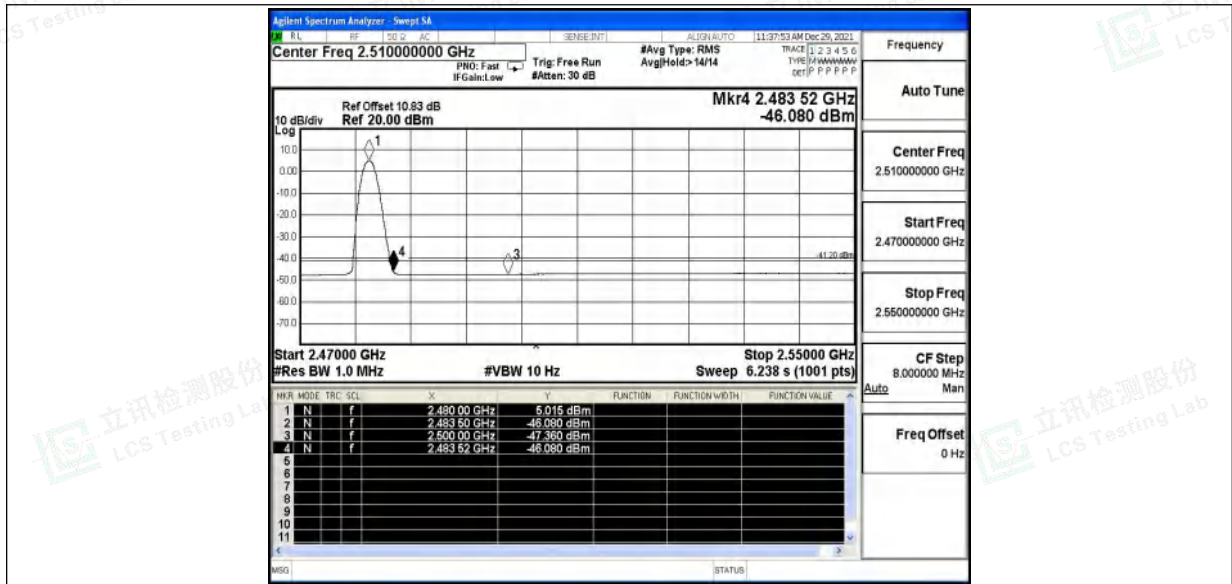
2DH5_Ant1_High_2480_Peak
