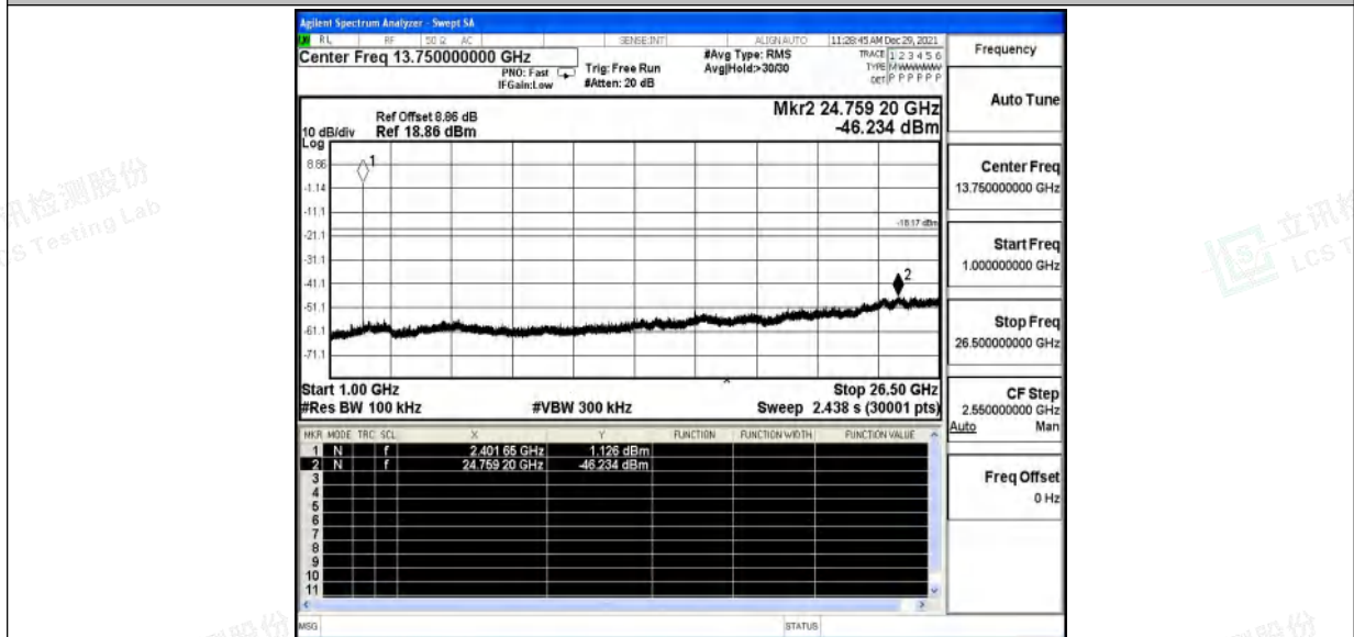
2DH5_Ant1_2441_0~Reference
