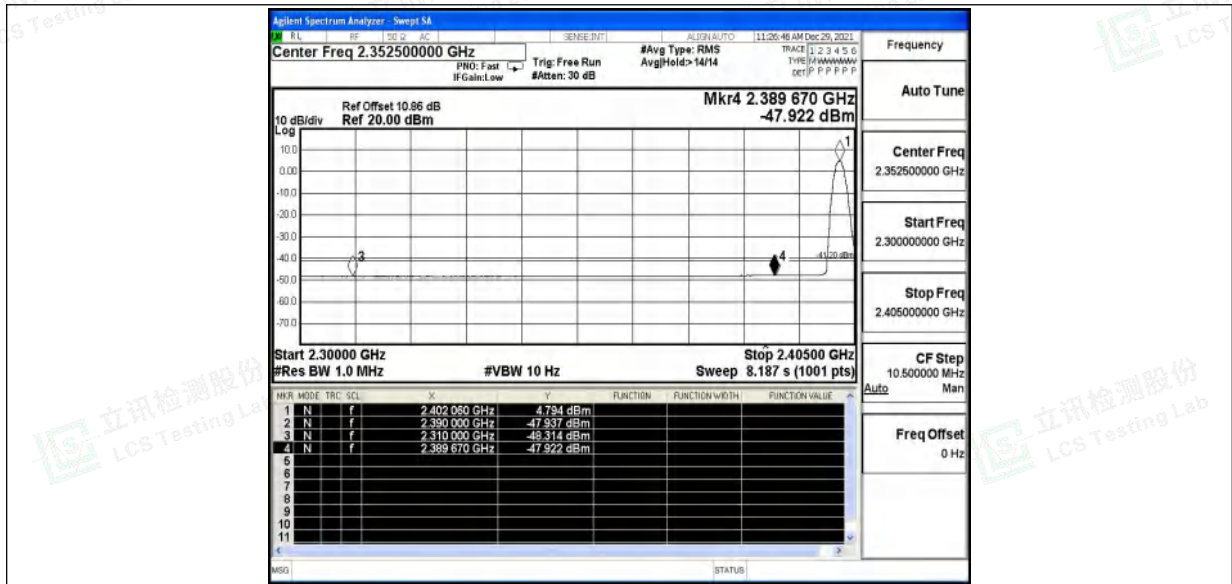
2DH5_Ant1_Low_2402_Peak
