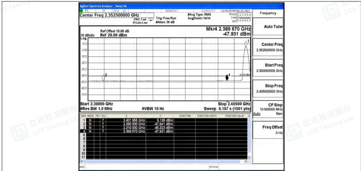
3DH5_Ant1_Low_2402_Peak
