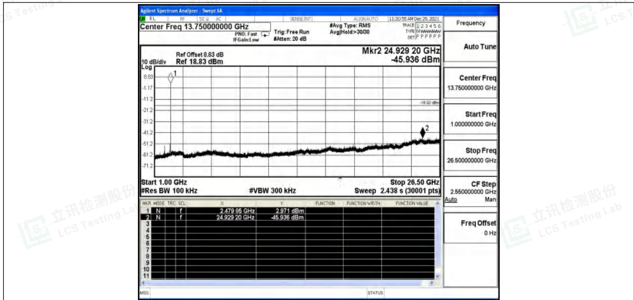
2DH5_Ant1_2402_0~Reference
