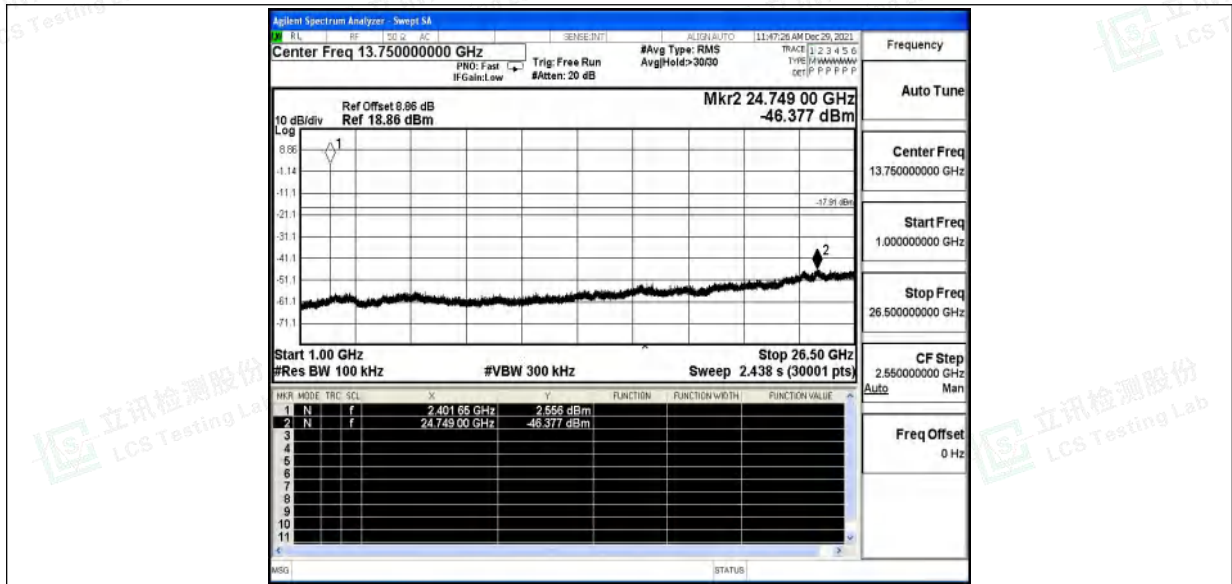
3DH5_Ant1_2441_0~Reference
