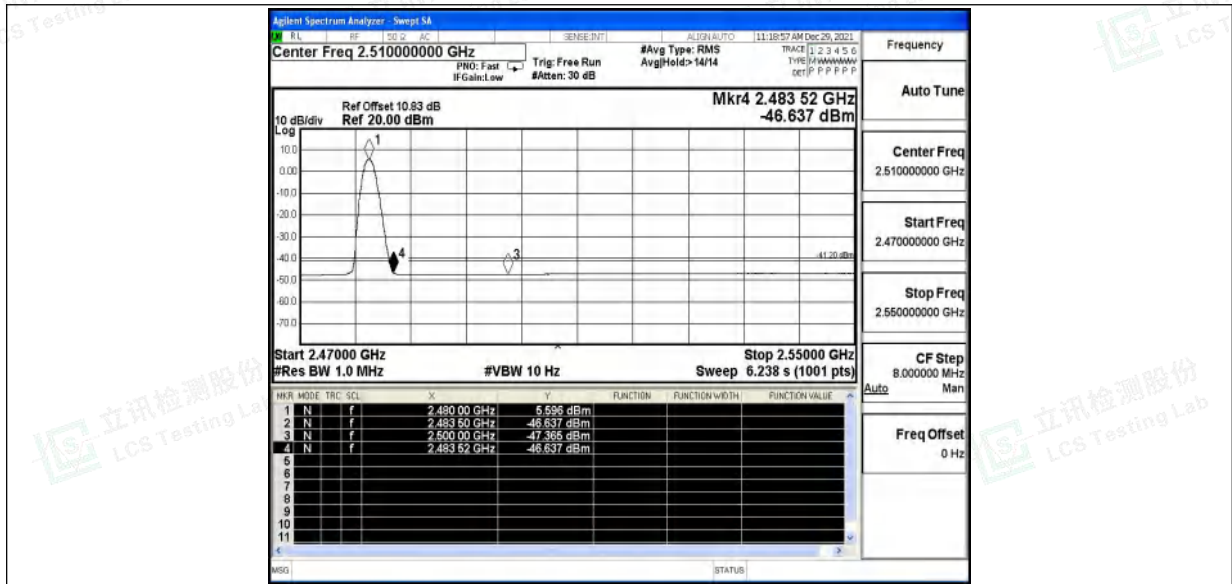
DH5_Ant1_High_2480_Peak
