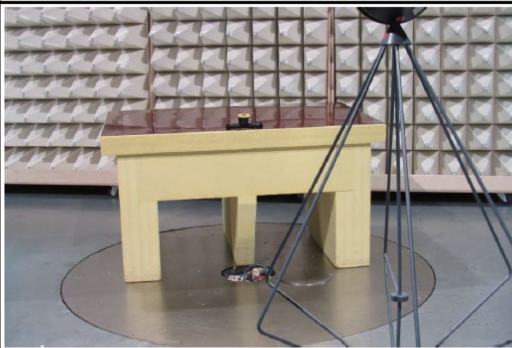
Radiated Setup 1
