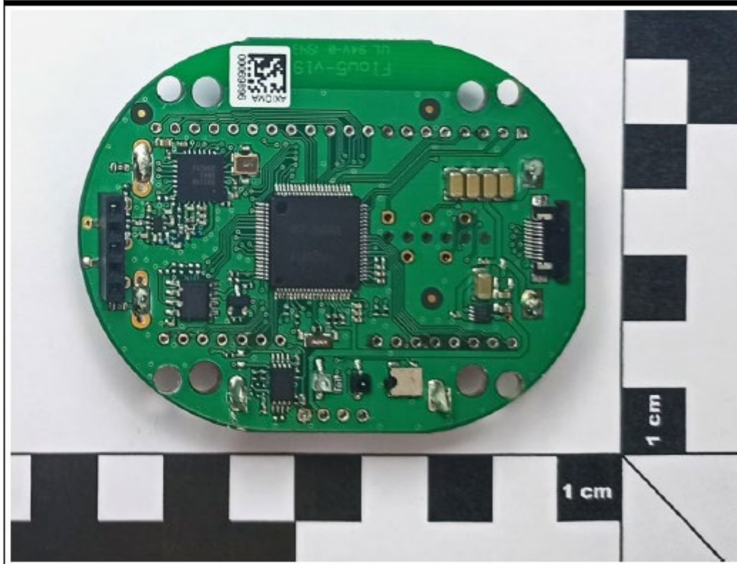
EUT PCB TOP SIDE WITHOU DISPLAY
