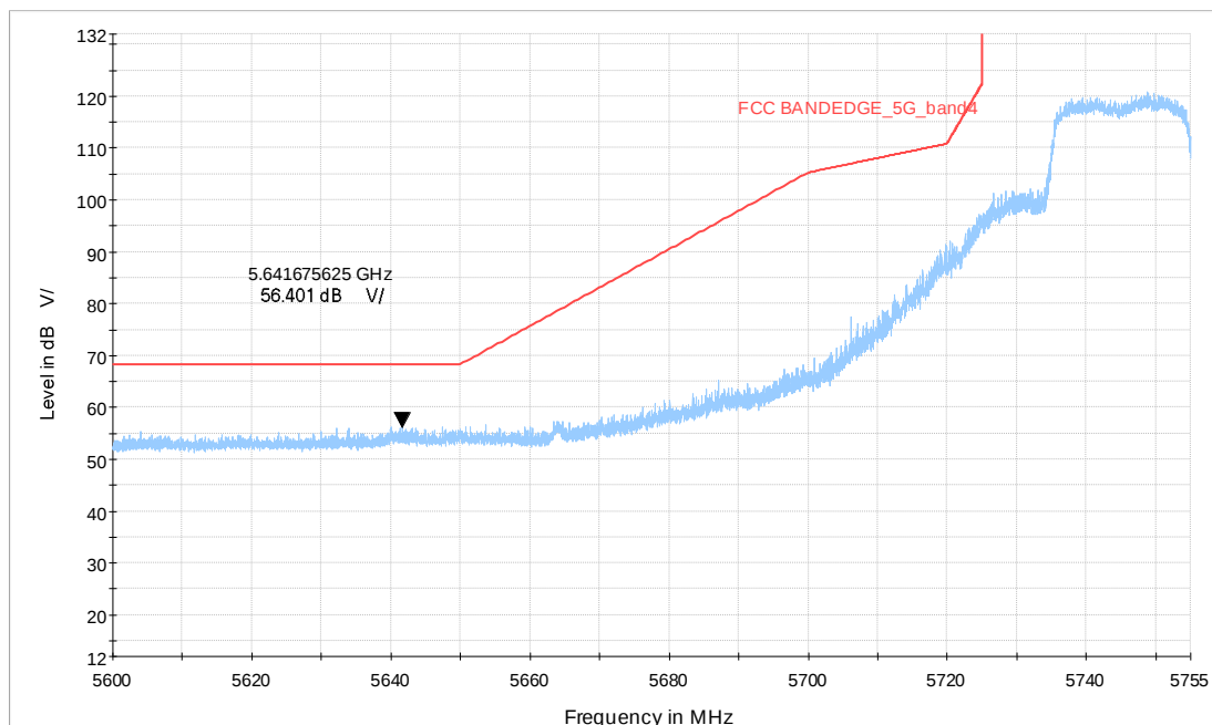
Wi-Fi 5G_ax20 CH149_5.6-5.755GHz_MCS0_MIMO_V_TP24
