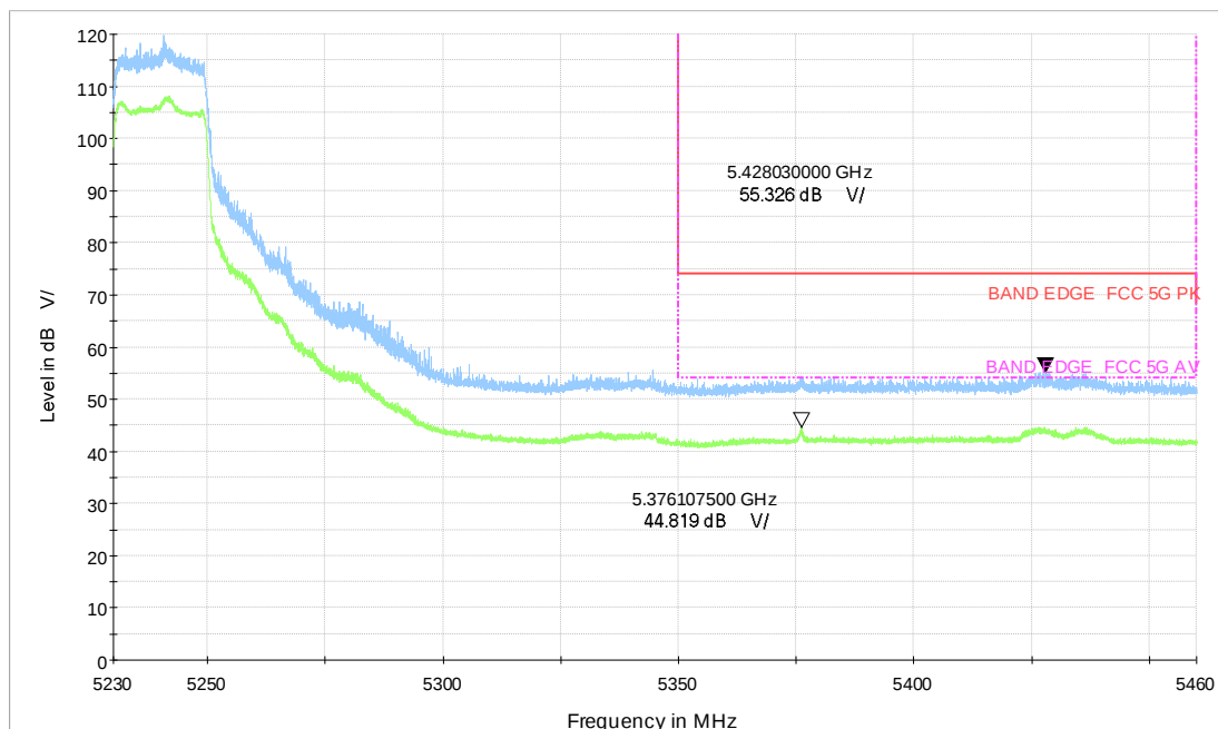
Wi-Fi 5G_ax20 CH48_5.23-5.46GHz_MCS0_MIMO_V_TP24
