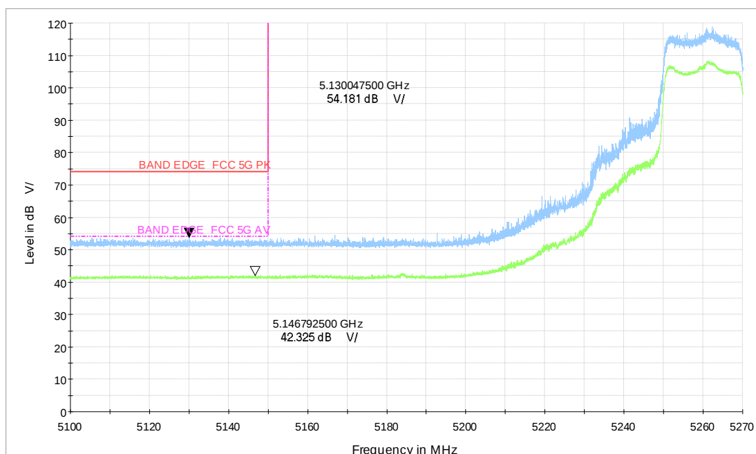
Wi-Fi 5G_ax20 CH52_5.1-5.27GHz_MCS0_MIMO_V_TP24
