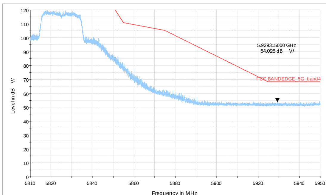
Wi-Fi 5G_ax20 CH165_5.81-5.95GHz_MCS0_MIMO_V_TP24
