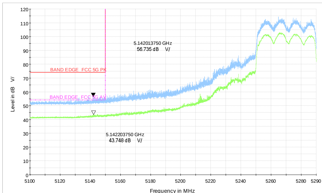
Wi-Fi 5G_ax40 CH54_5.1-5.29GHz_MCS0_MIMO_V_TP24
