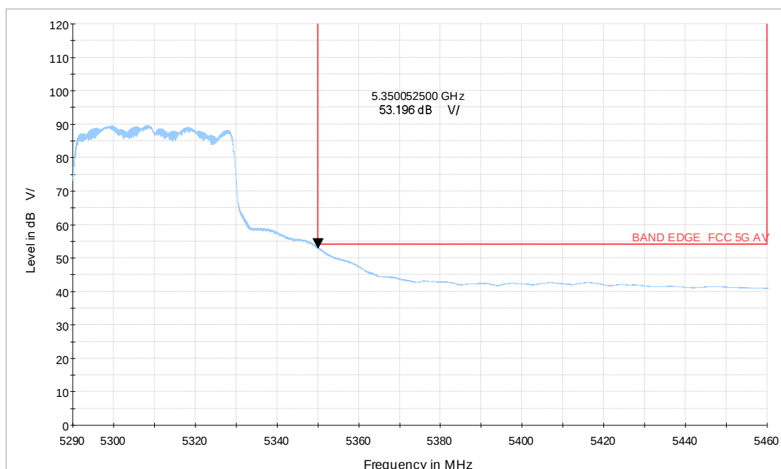
Wi-Fi 5G_ax40 CH62_5.29-5.46GHz_MCS0_MIMO_V_TP22_AV
