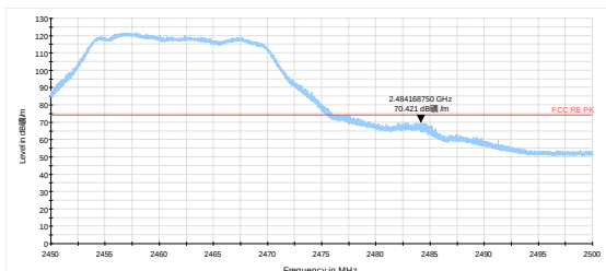
802.11g-Channel 11 Peak
