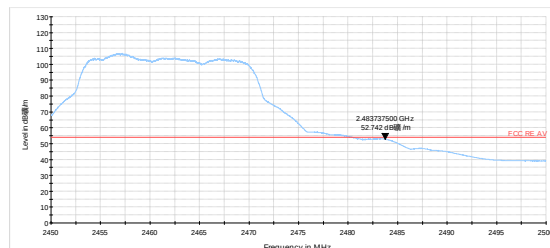
802.11g-Channel 11 Average
