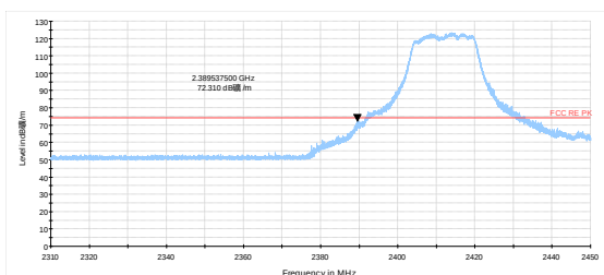
802.11g-Channel 1 Peak
