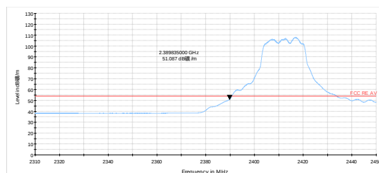
802.11g-Channel 1 Average
