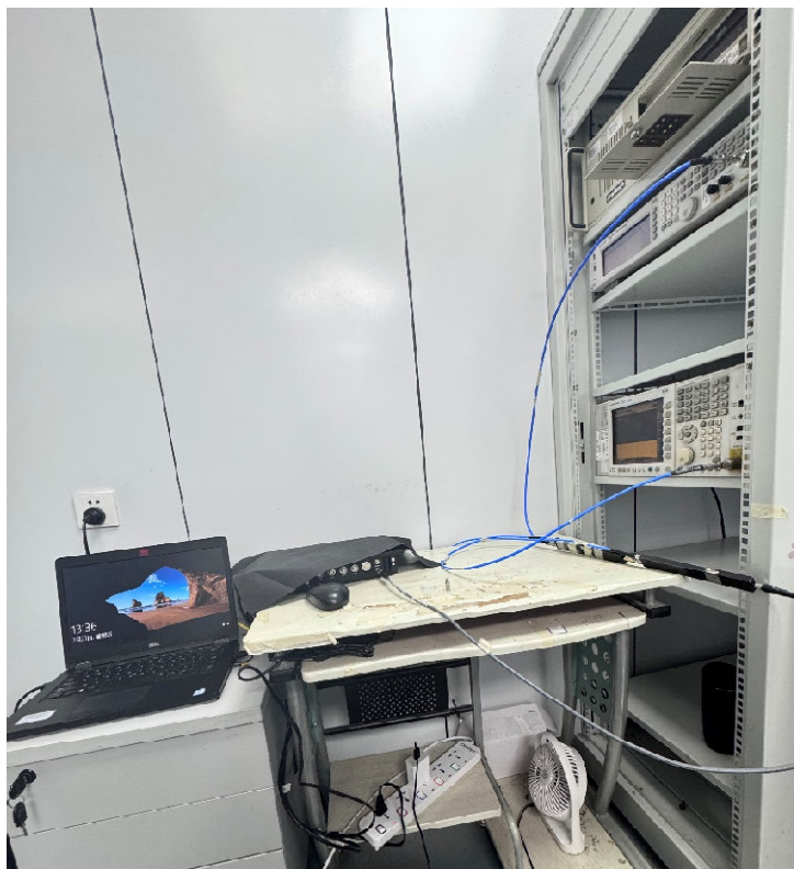
Picture 1 DFS Test Setup
