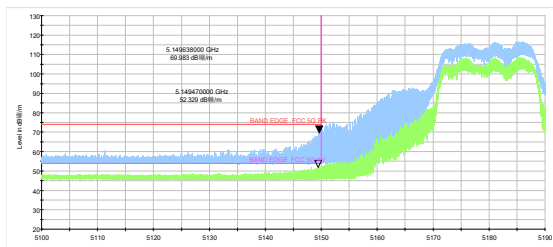
802.11a-Channel 36: Peak & Average
