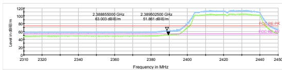
802.11n HT40 -Channel 3 Peak+ Average
