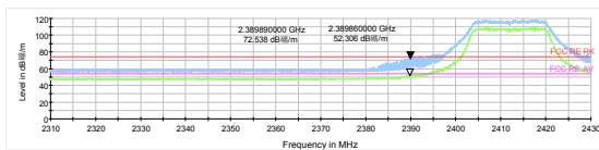
802.11g-Channel 1 Peak+ Average
