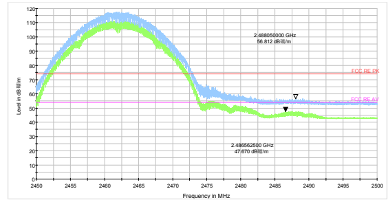
802.11b-Channel 11 Peak+ Average
