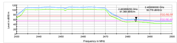
802.11n HT40 -Channel 9 Peak+ Average
