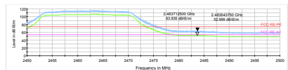
802.11n HT20 -Channel 11 Peak+ Average
