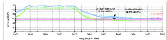
802.11g-Channel 11 Peak+ Average
