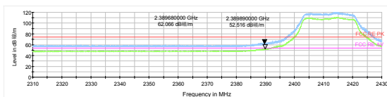
802.11n HT20 -Channel 1 Peak+ Average
