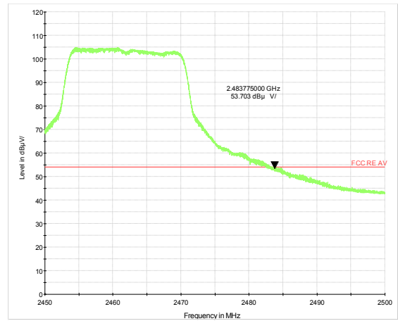
802.11g-Channel 11 Average
