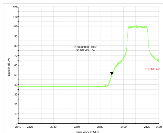
802.11g-Channel 1 Average
