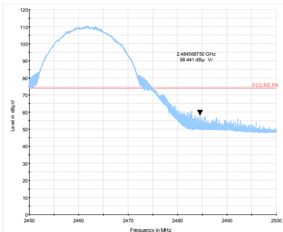
802.11b-Channel 11 Peak
