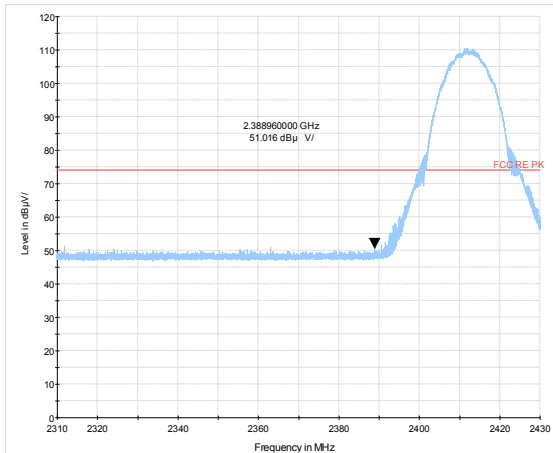
802.11b-Channel 1 Peak
