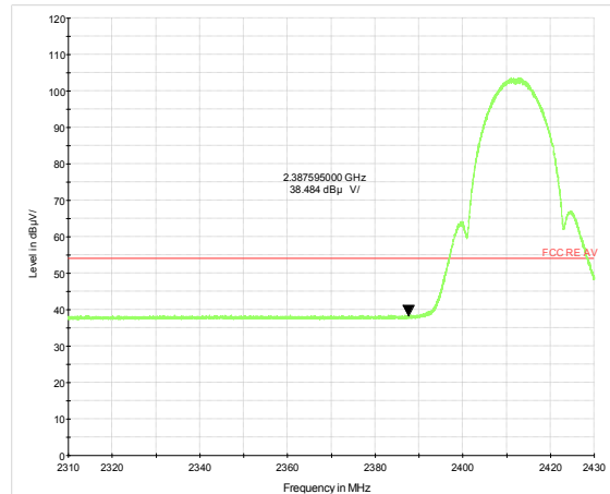
802.11b-Channel 1 Average
