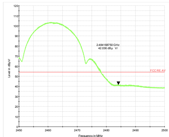
802.11b-Channel 11 Average
