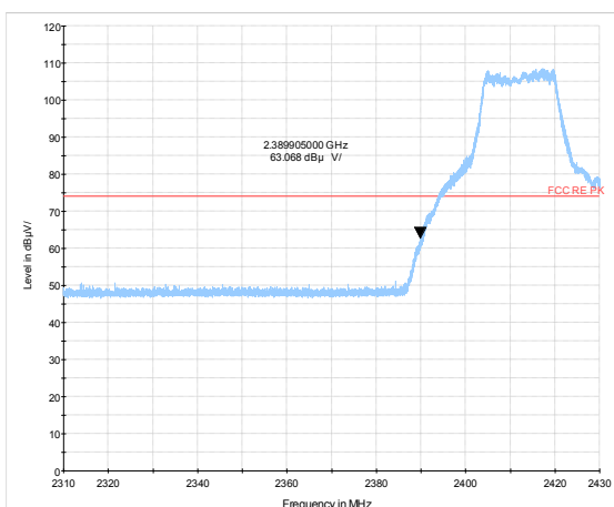
802.11g-Channel 1 Peak
