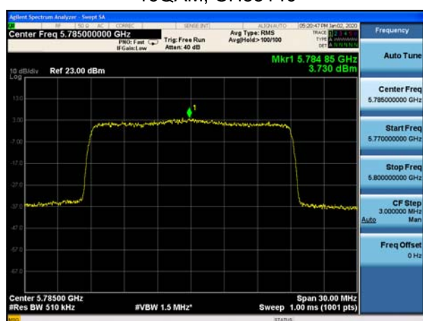
16QAM, CH53540
