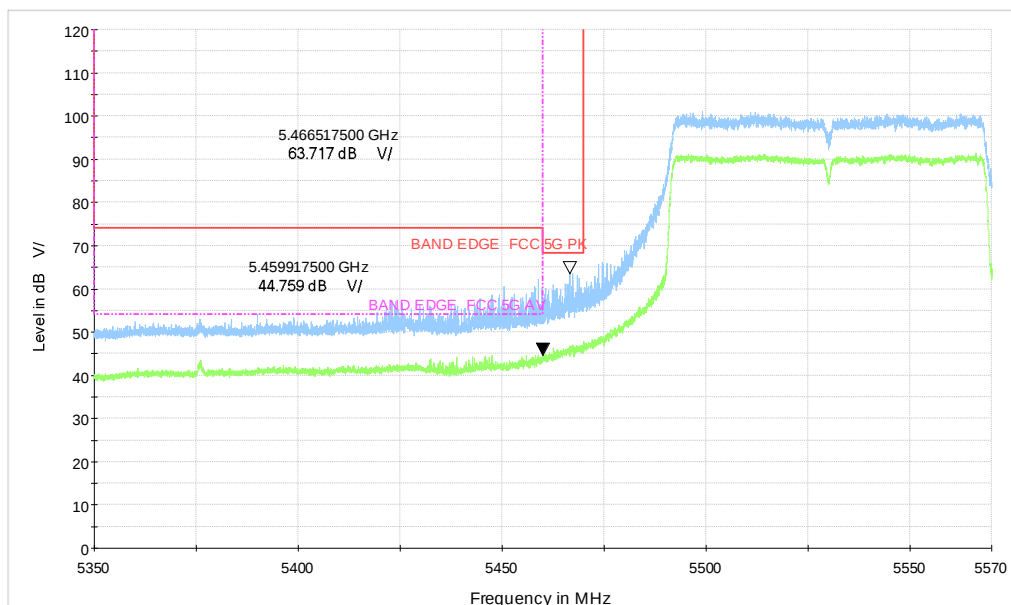
5GWIFI_ac80_CH106_5.35-5.57GHz_MCS0_H
