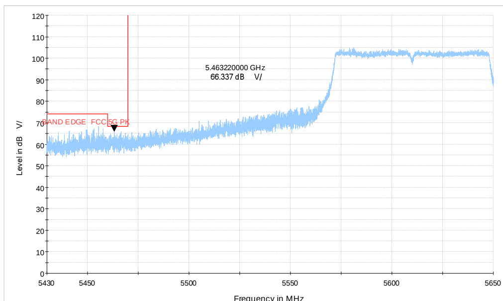
5GWIFI_ac80_CH122_5.43-5.65GHz_MCS0H
