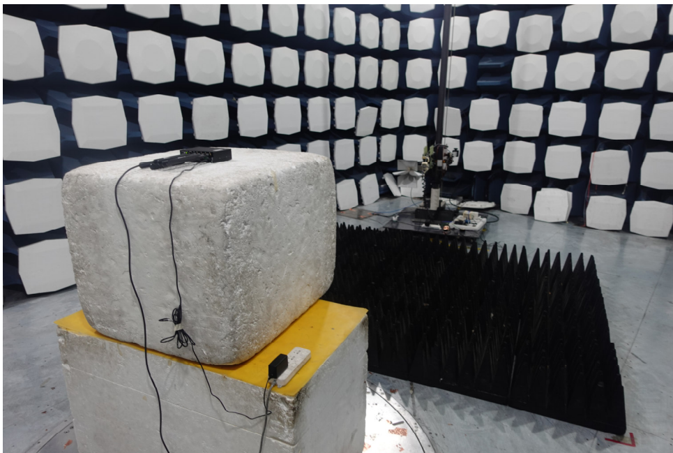
Picture 1: Radiated Spurious Emissions Test setup
