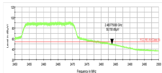
802.11g-Channel 11 Average
