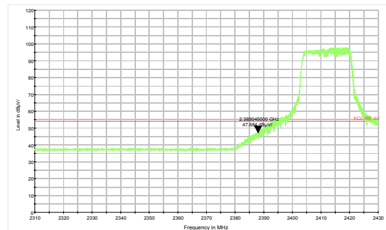
802.11g-Channel 1 Average
