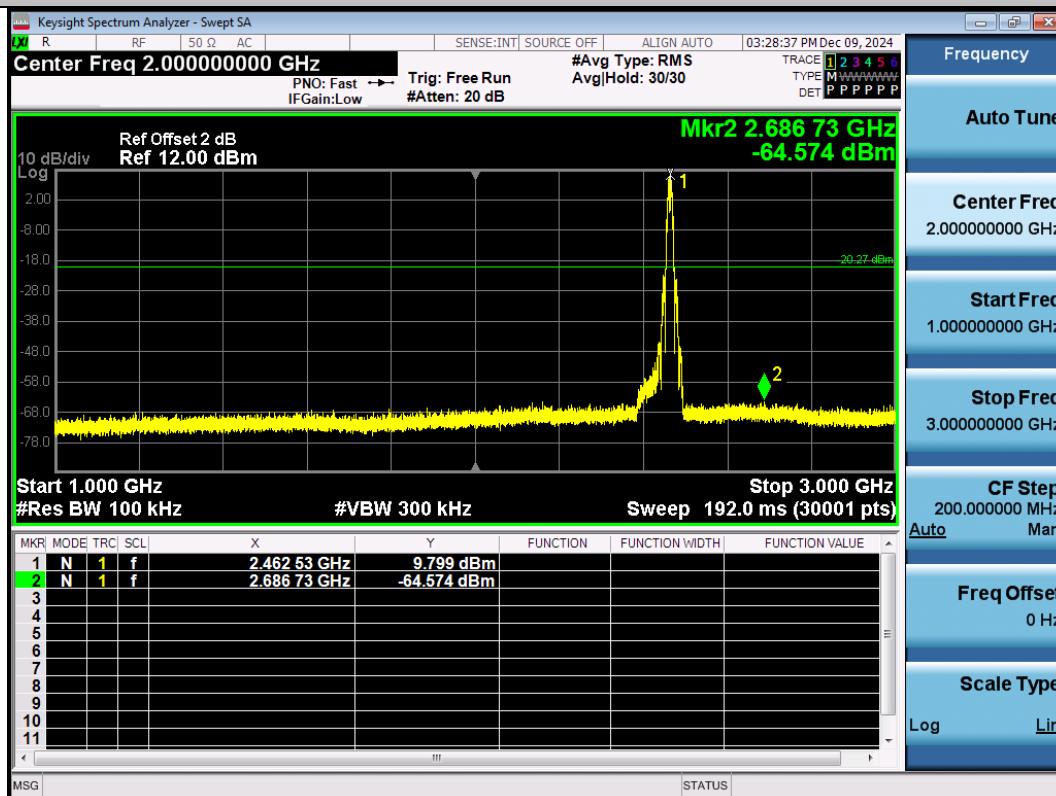
11B-Ant1-2462-1000~3000-PASS
