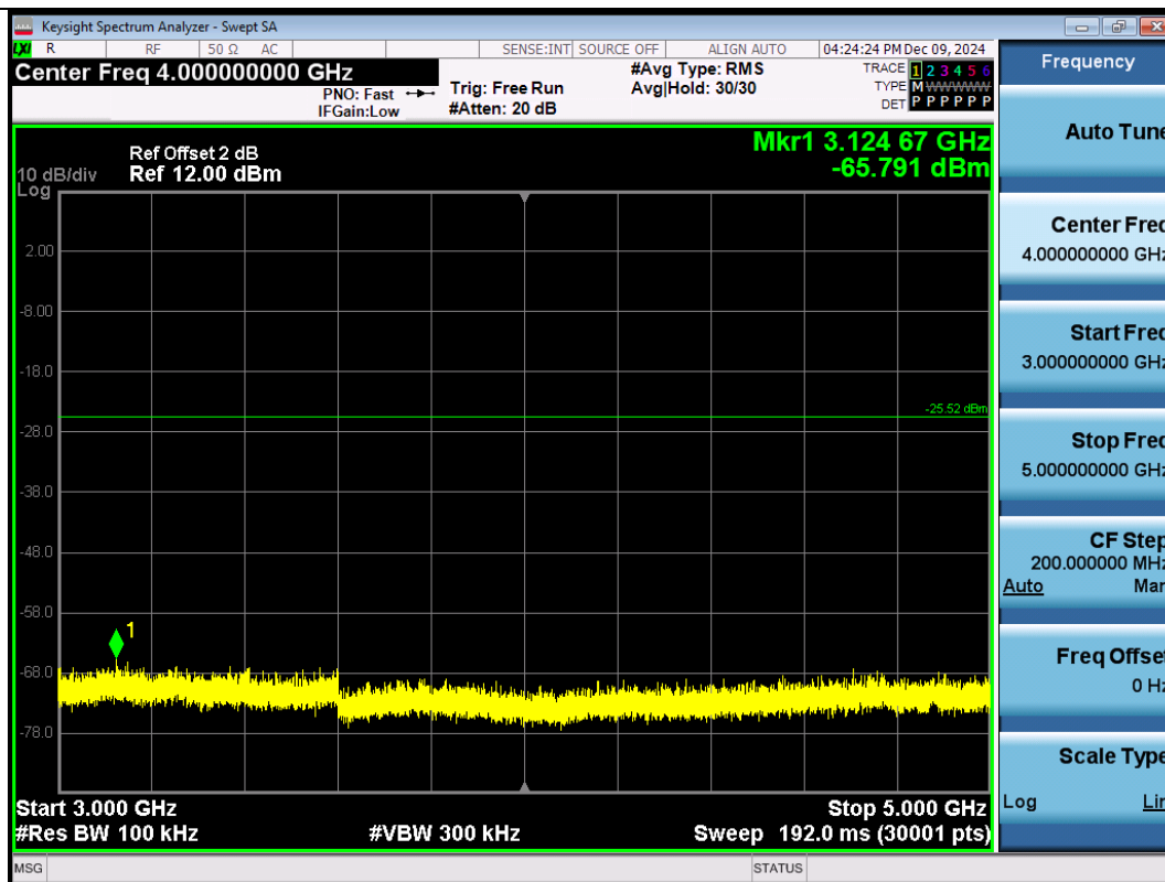
11G-Ant1-2437-3000~5000-PASS
