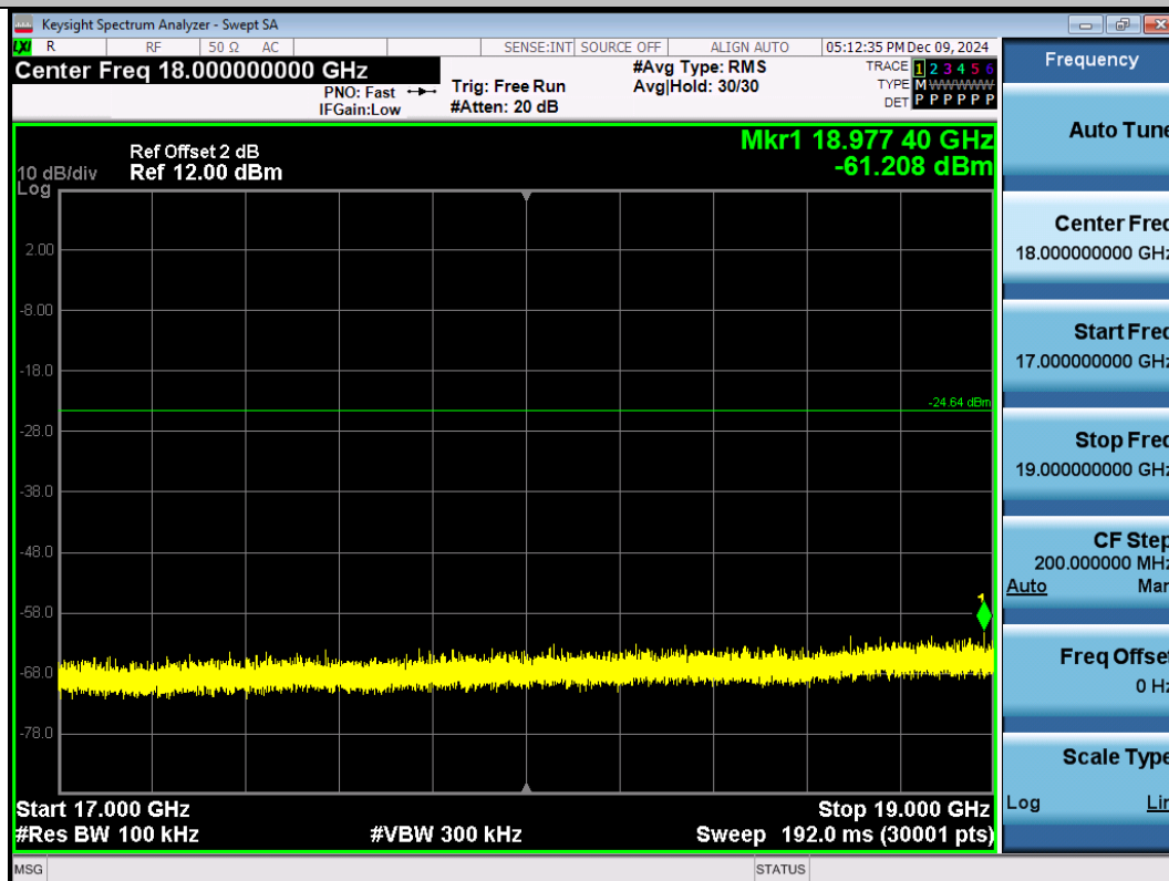
11N20SISO-Ant1-2412-17000~19000-PASS
