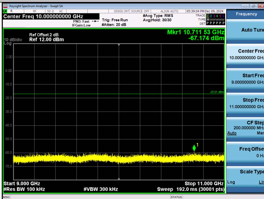
11N20SISO-Ant1-2462-9000~11000-PASS
