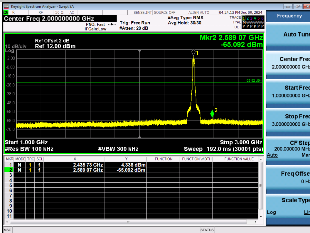
11G-Ant1-2437-1000~3000-PASS
