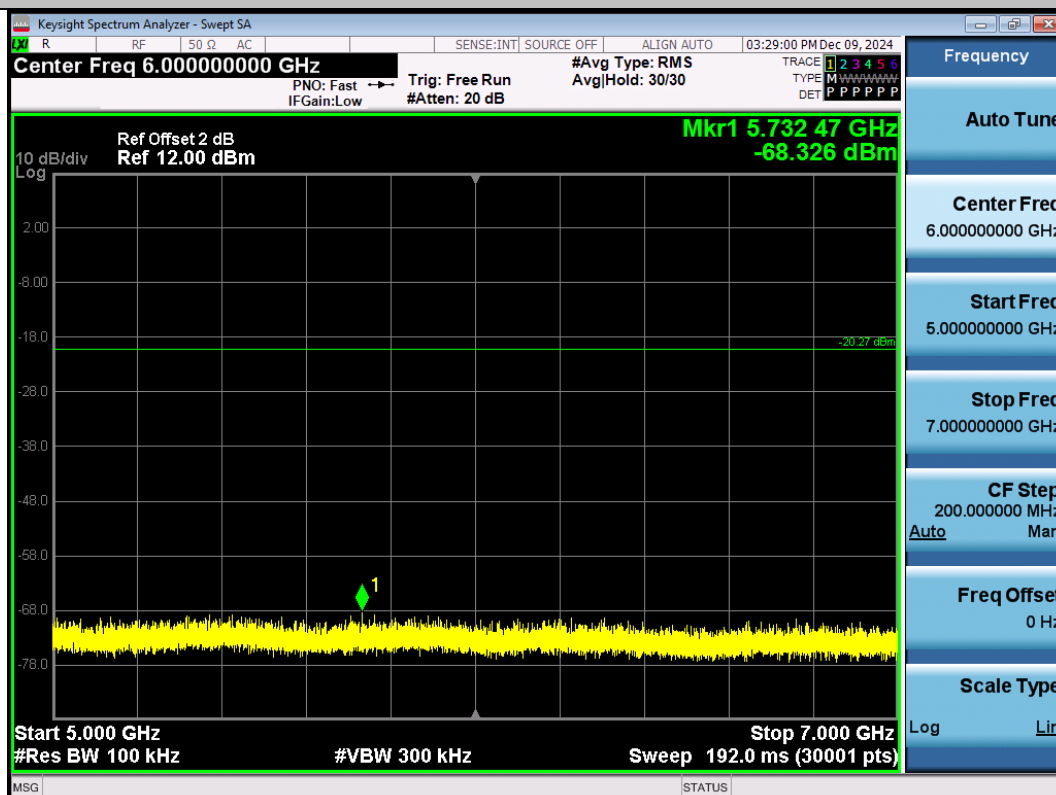
11B-Ant1-2462-5000-7000-PASS
