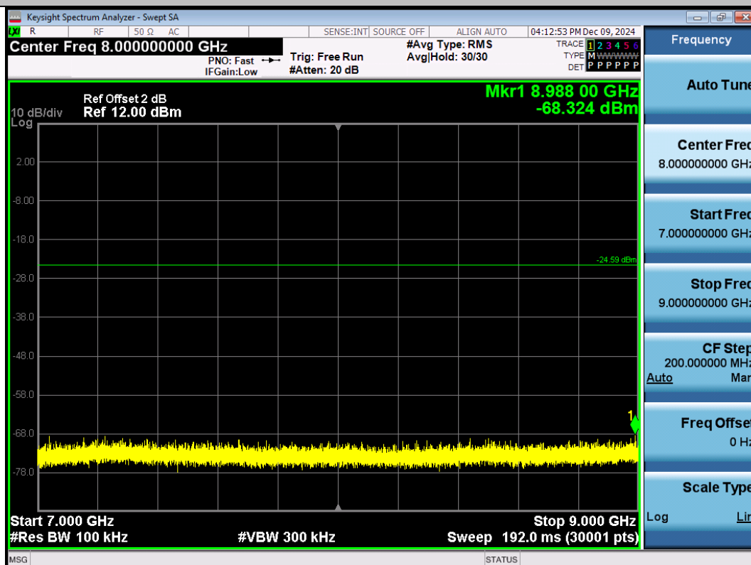
11G-Ant1-2412-7000-9000-PASS
