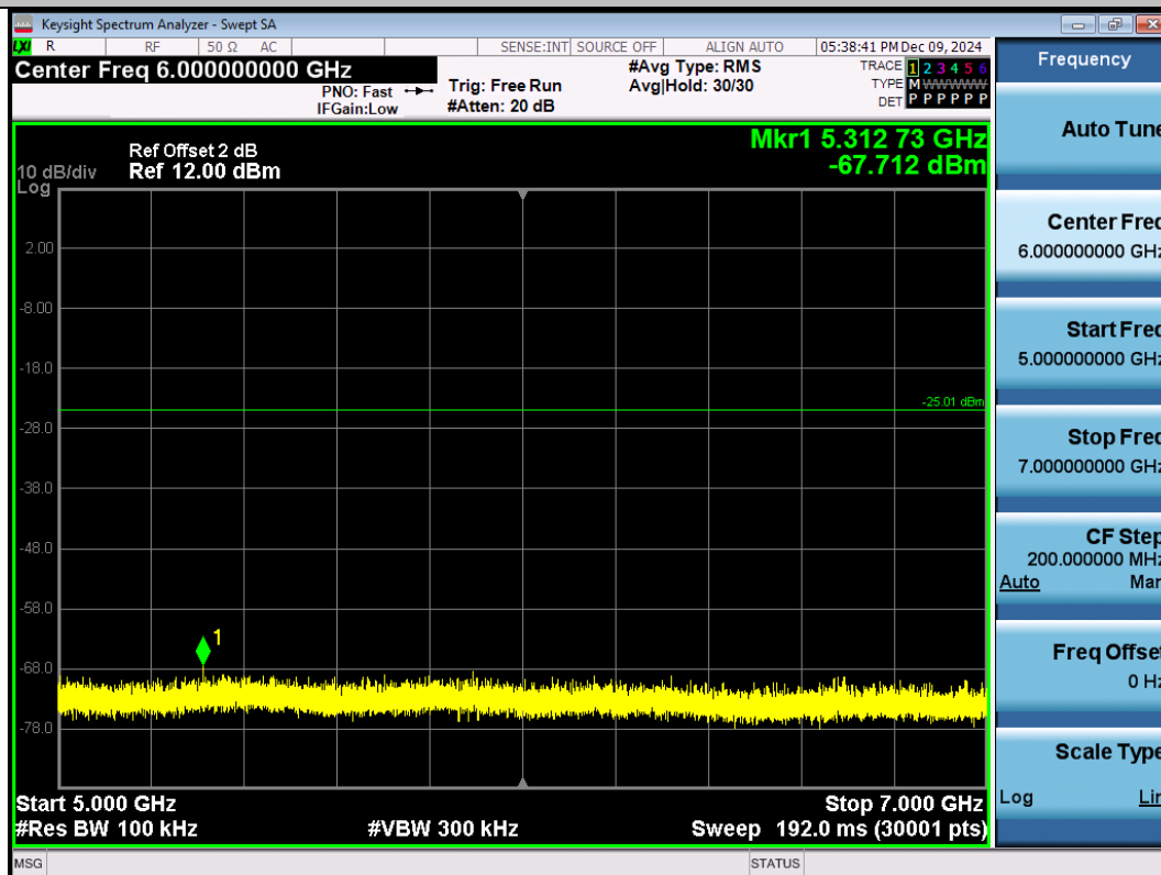
11N20SISO-Ant1-2462-5000~7000-PASS
