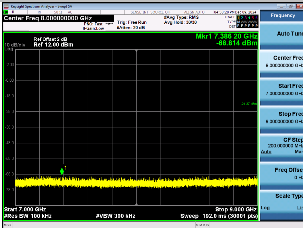
11G-Ant1-2462-7000-9000-PASS
