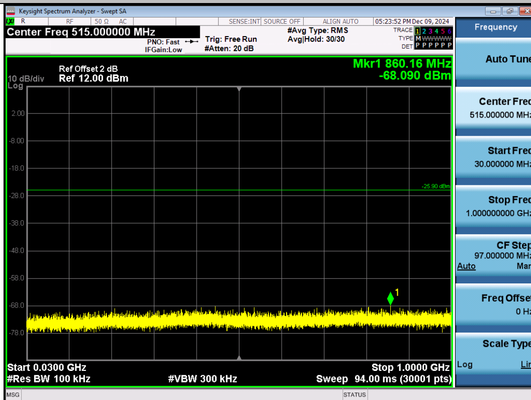
11N20SISO-Ant1-2437-30~1000-PASS
