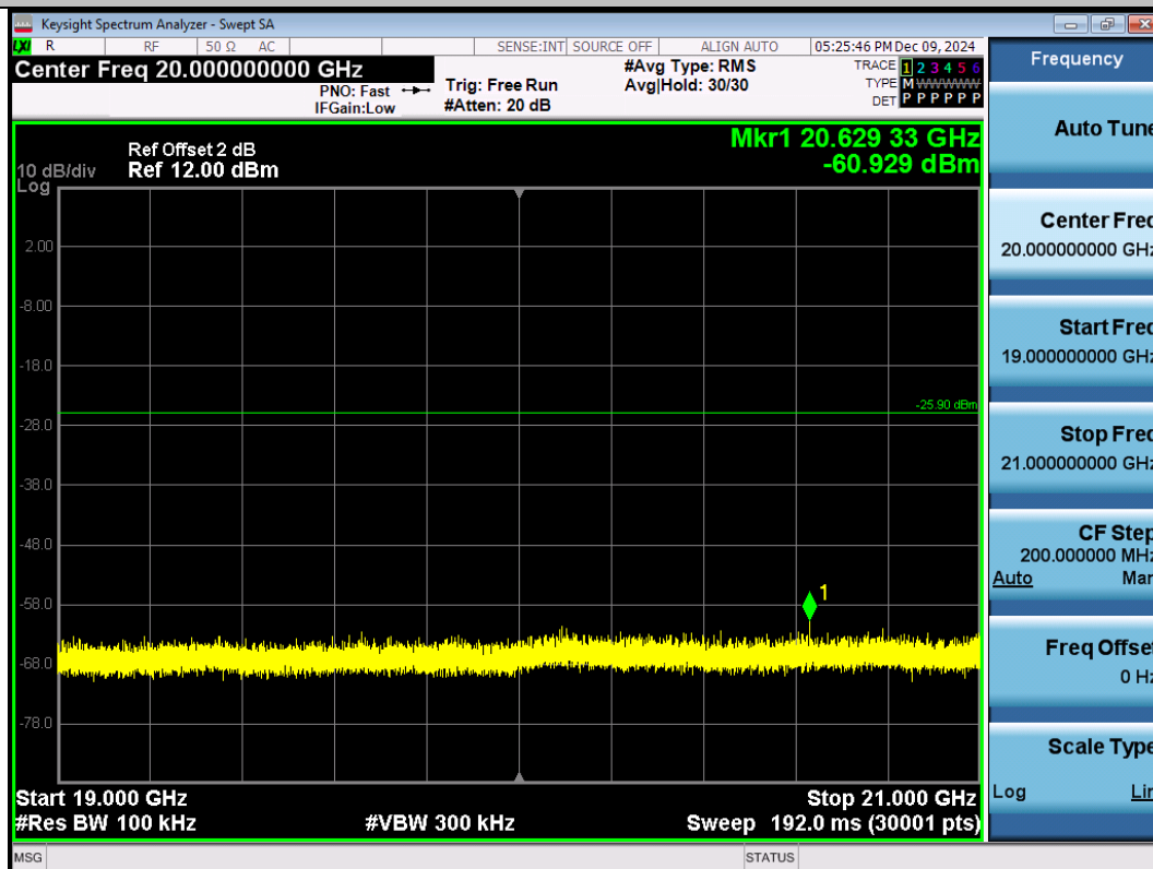
11N20SISO-Ant1-2437-19000~21000-PASS
