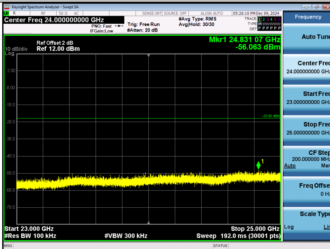
11N20SISO-Ant1-2437-23000~25000-PASS
