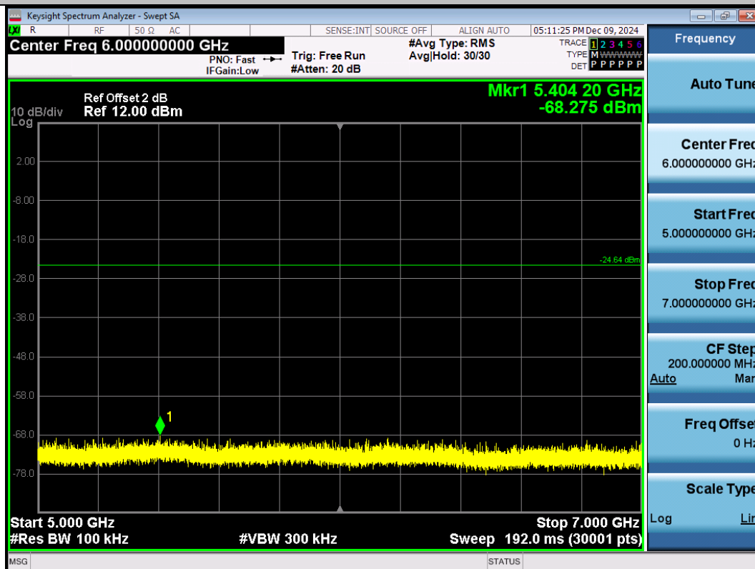
11N20SISO-Ant1-2412-5000~7000-PASS
