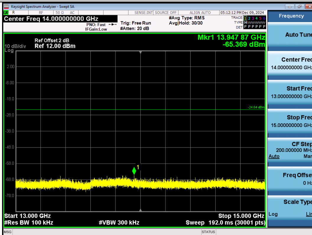
11N20SISO-Ant1-2412-13000~15000-PASS
