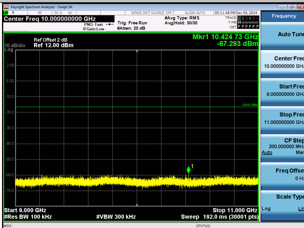
11N20SISO-Ant1-2412-9000~11000-PASS
