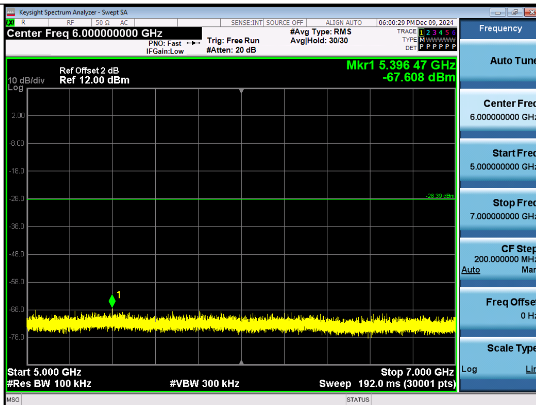
11N40SISO-Ant1-2422-5000~7000-PASS
