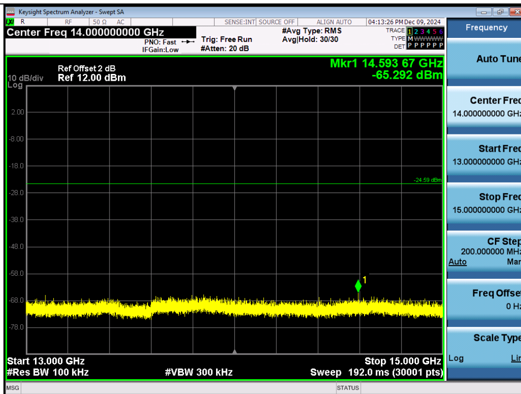
11G-Ant1-2412-13000~15000-PASS
