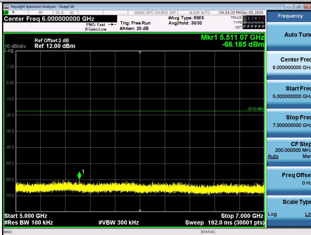
11G-Ant1-2437-5000~7000-PASS
