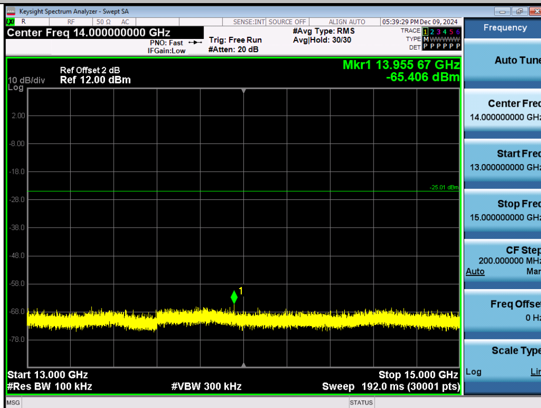
11N20SISO-Ant1-2462-13000~15000-PASS
