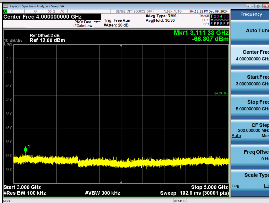
11G-Ant1-2412-3000~5000-PASS
