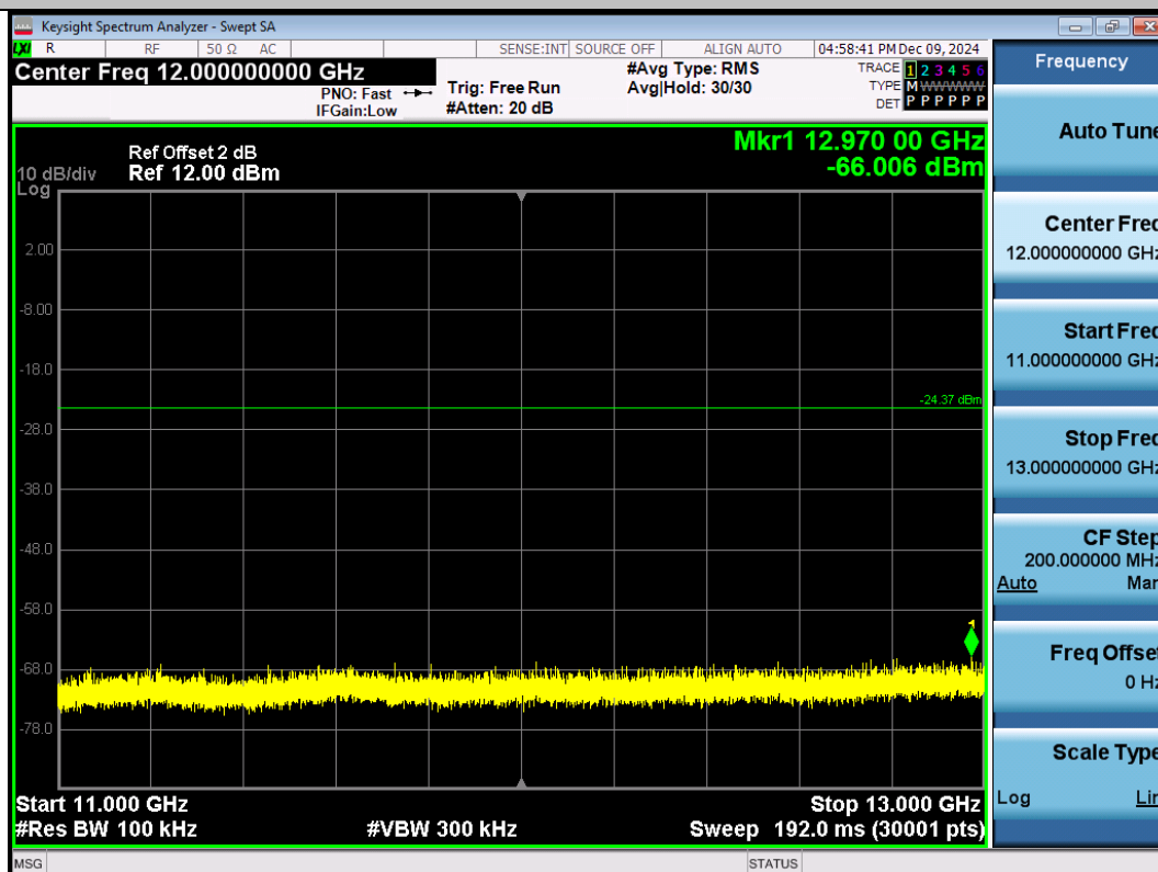
11G-Ant1-2462-11000~13000-PASS
