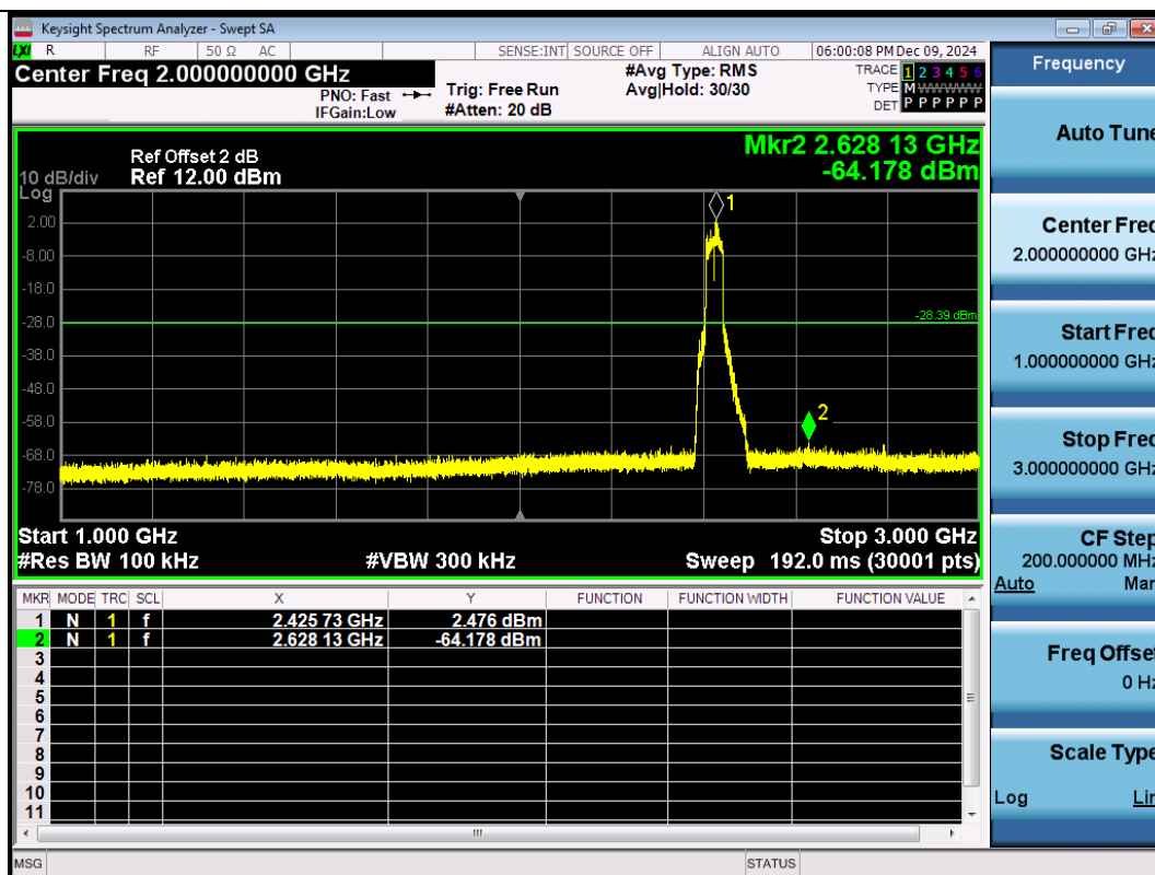
11N40SISO-Ant1-2422-1000~3000-PASS
