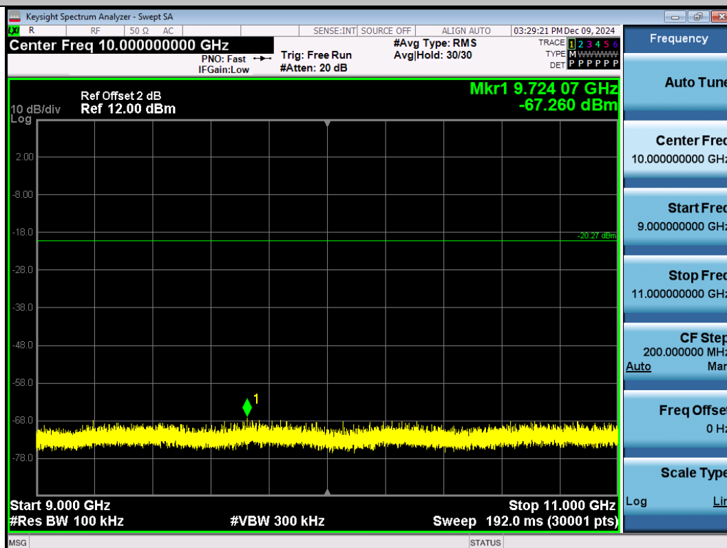
11B-Ant1-2462-9000~11000-PASS
