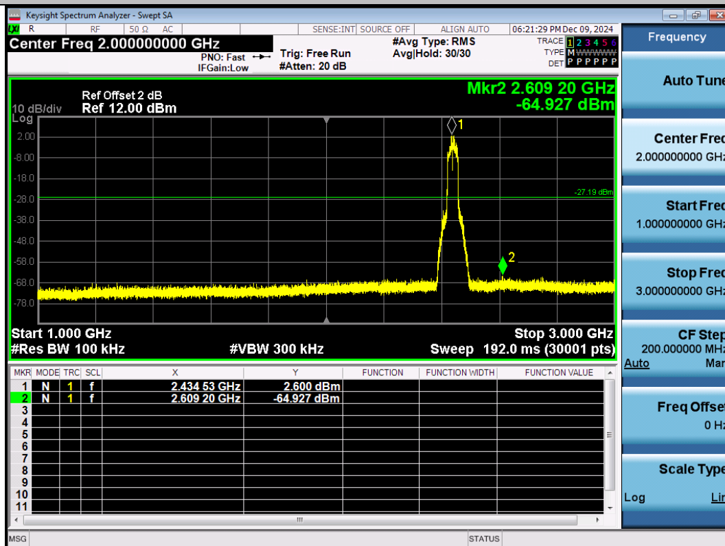
11N40SISO-Ant1-2437-1000~3000-PASS
