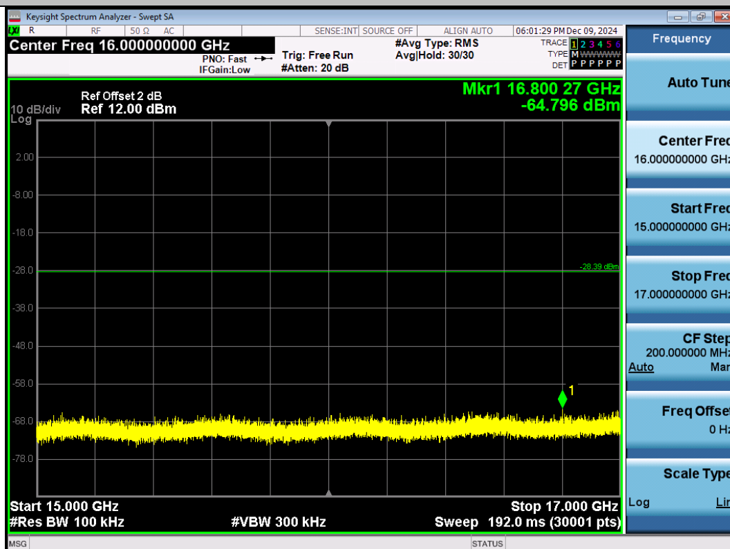
11N40SISO-Ant1-2422-15000~17000-PASS
