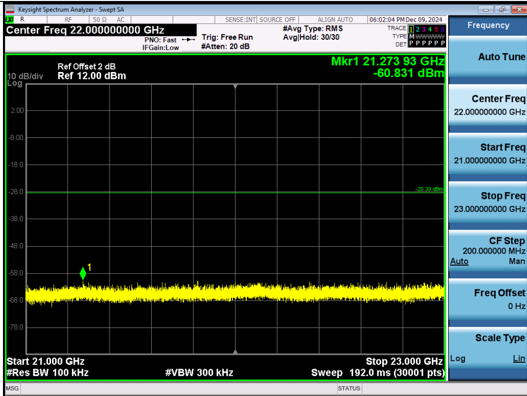
11N40SISO-Ant1-2422-21000~23000-PASS
