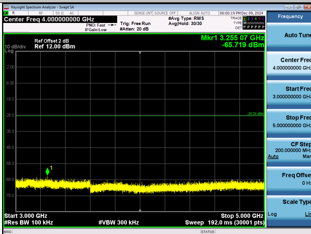
11N40SISO-Ant1-2422-3000~5000-PASS
