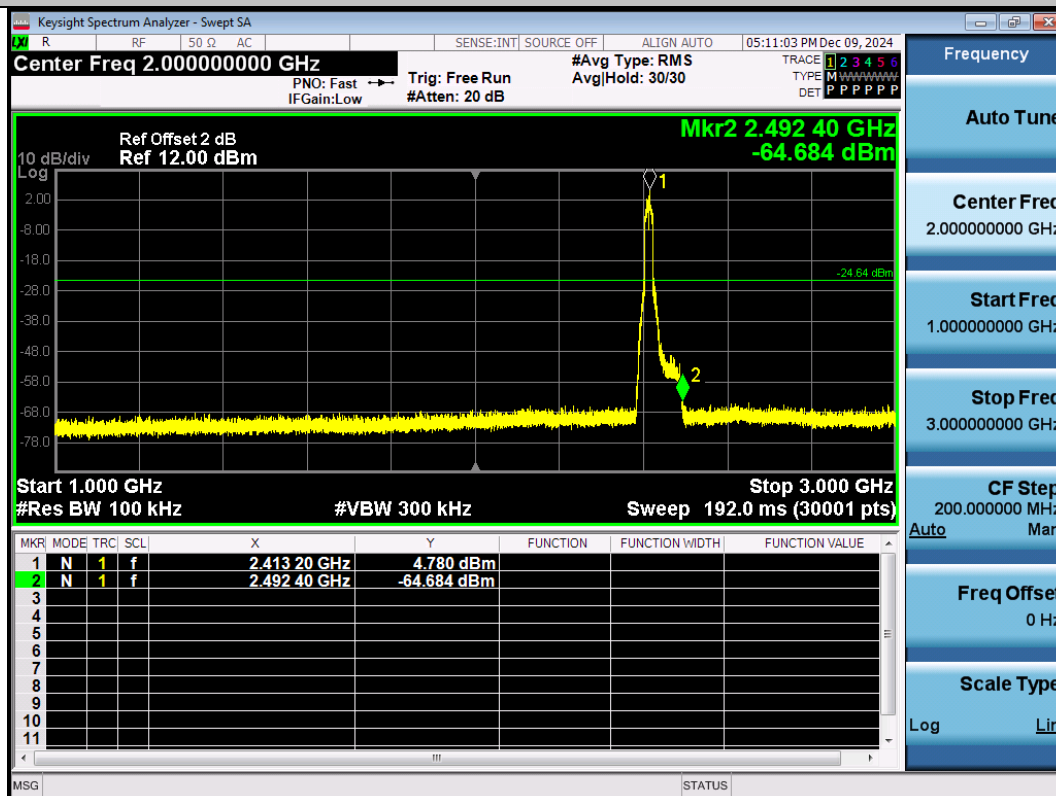
11N20SISO-Ant1-2412-1000~3000-PASS
