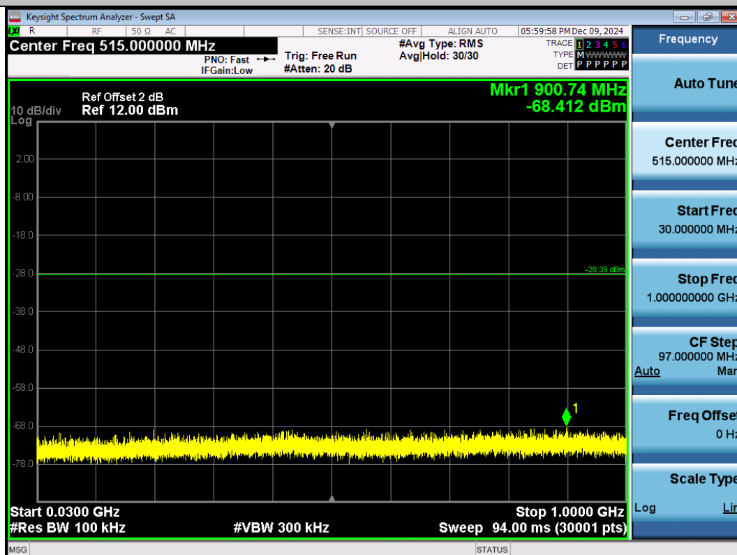
11N40SISO-Ant1-2422-30~1000-PASS
