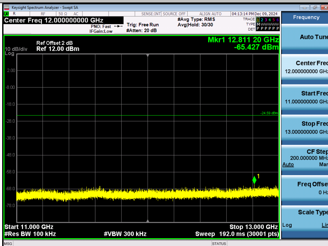
11G-Ant1-2412-11000~13000-PASS
