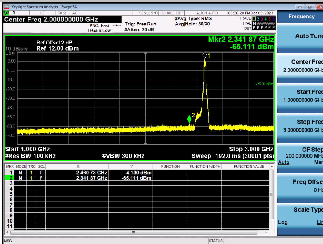
11N20SISO-Ant1-2462-1000~3000-PASS
