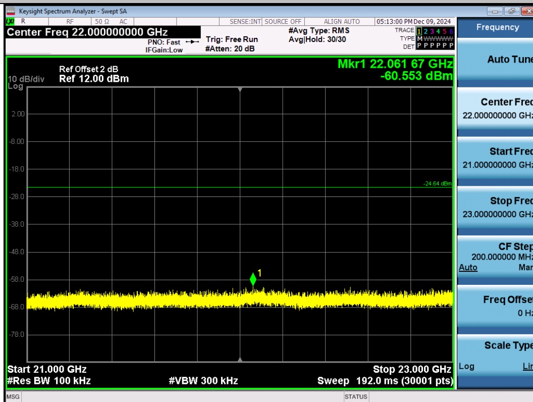
11N20SISO-Ant1-2412-21000~23000-PASS
