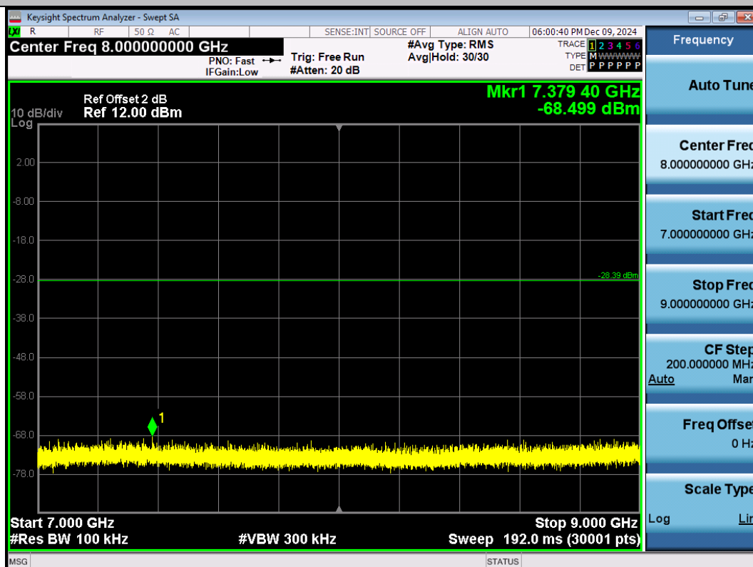
11N40SISO-Ant1-2422-7000~9000-PASS
