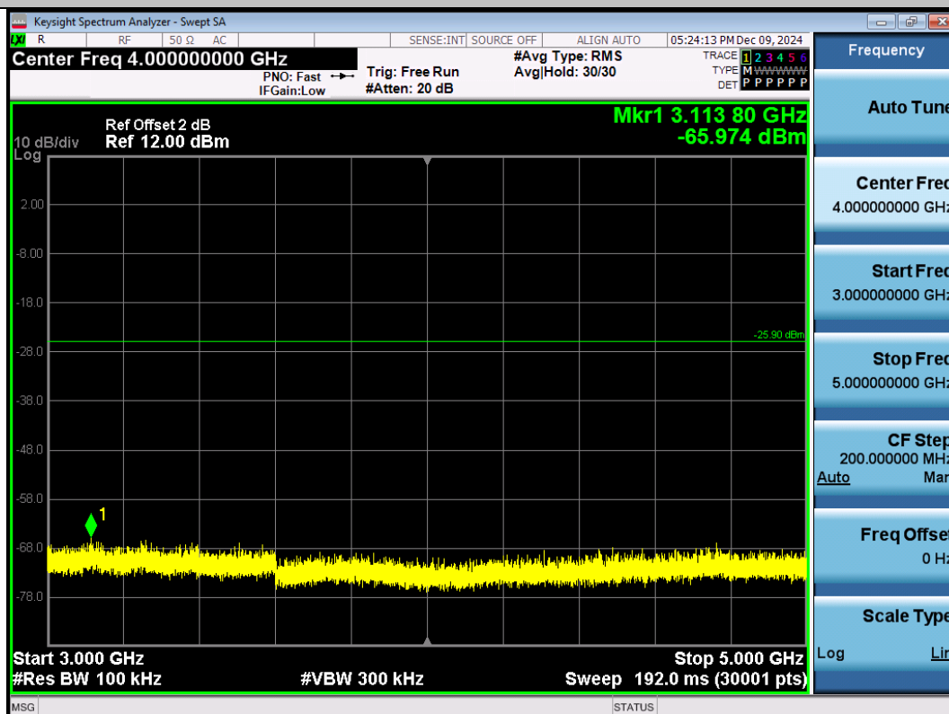
11N20SISO-Ant1-2437-3000~5000-PASS
