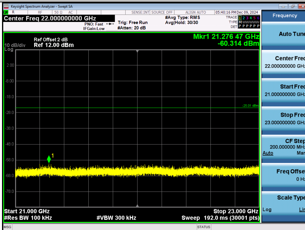
11N20SISO-Ant1-2462-21000~23000-PASS
