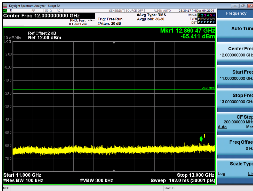
11N20SISO-Ant1-2462-11000~13000-PASS
