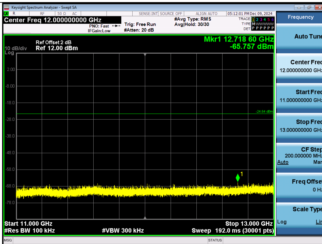
11N20SISO-Ant1-2412-11000~13000-PASS
