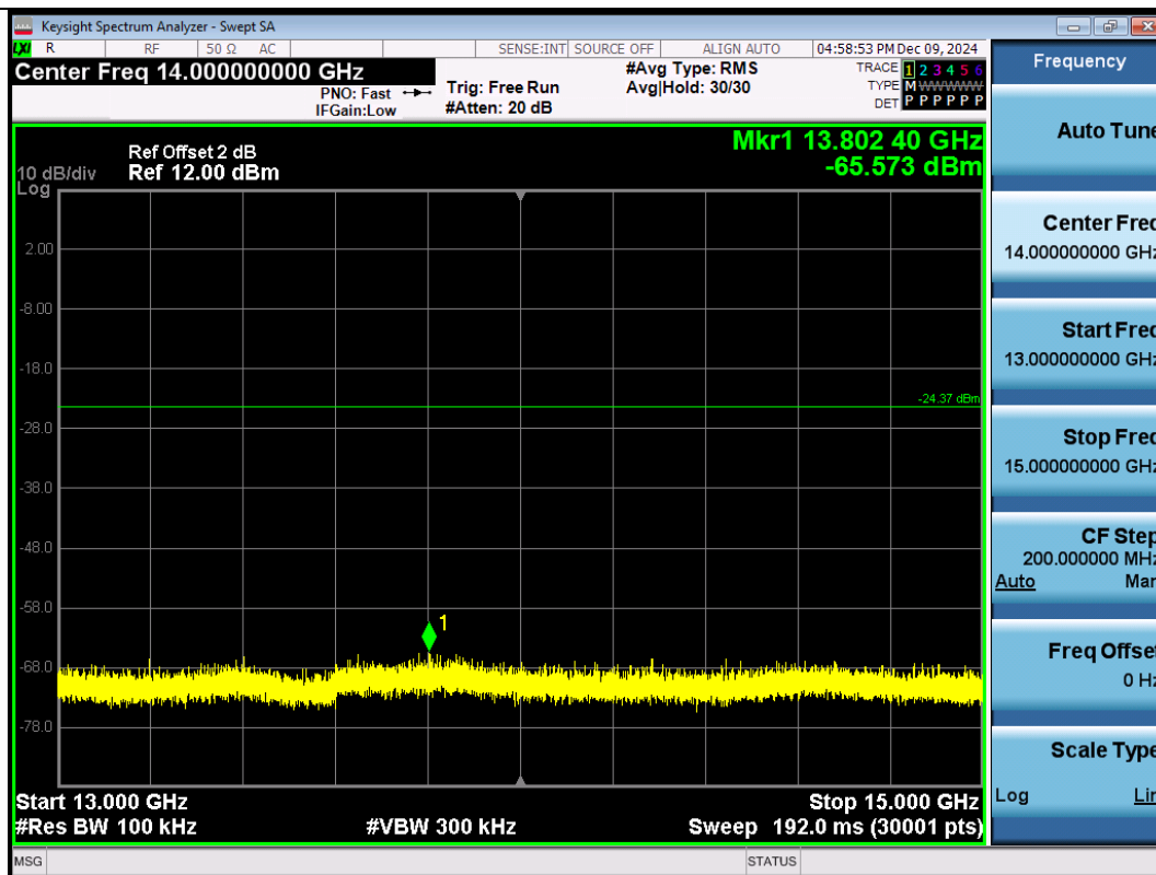
11G-Ant1-2462-13000~15000-PASS
