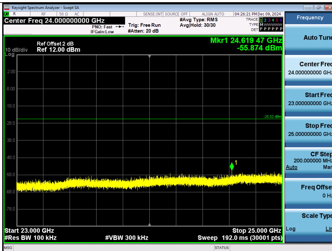
11G-Ant1-2437-23000~25000-PASS
