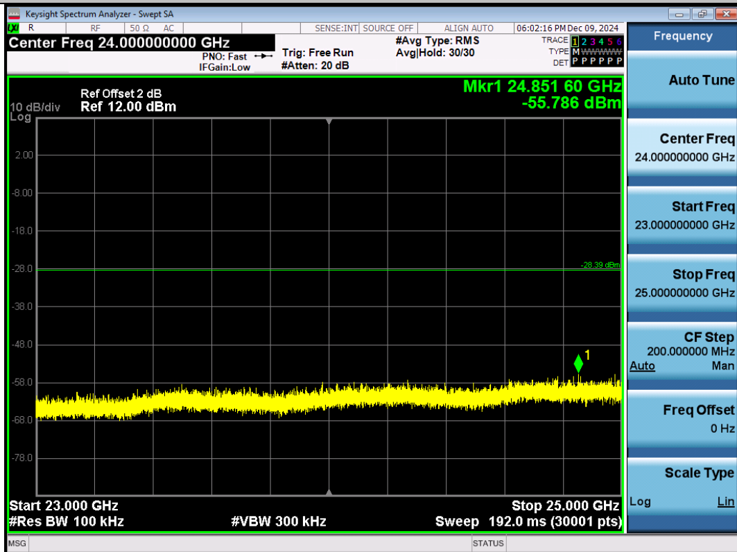
11N40SISO-Ant1-2422-23000~25000-PASS
