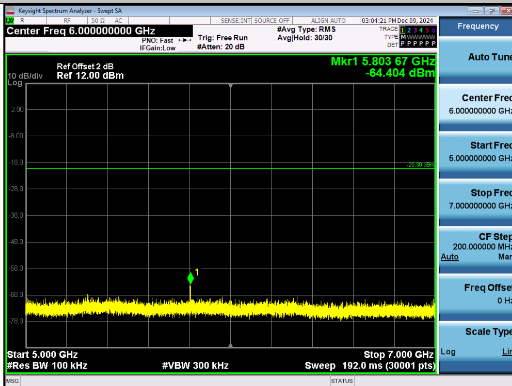
11B-Ant1-2412-5000-7000-PASS
