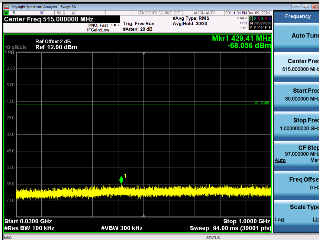
11B-Ant1-2437-30~1000-PASS
