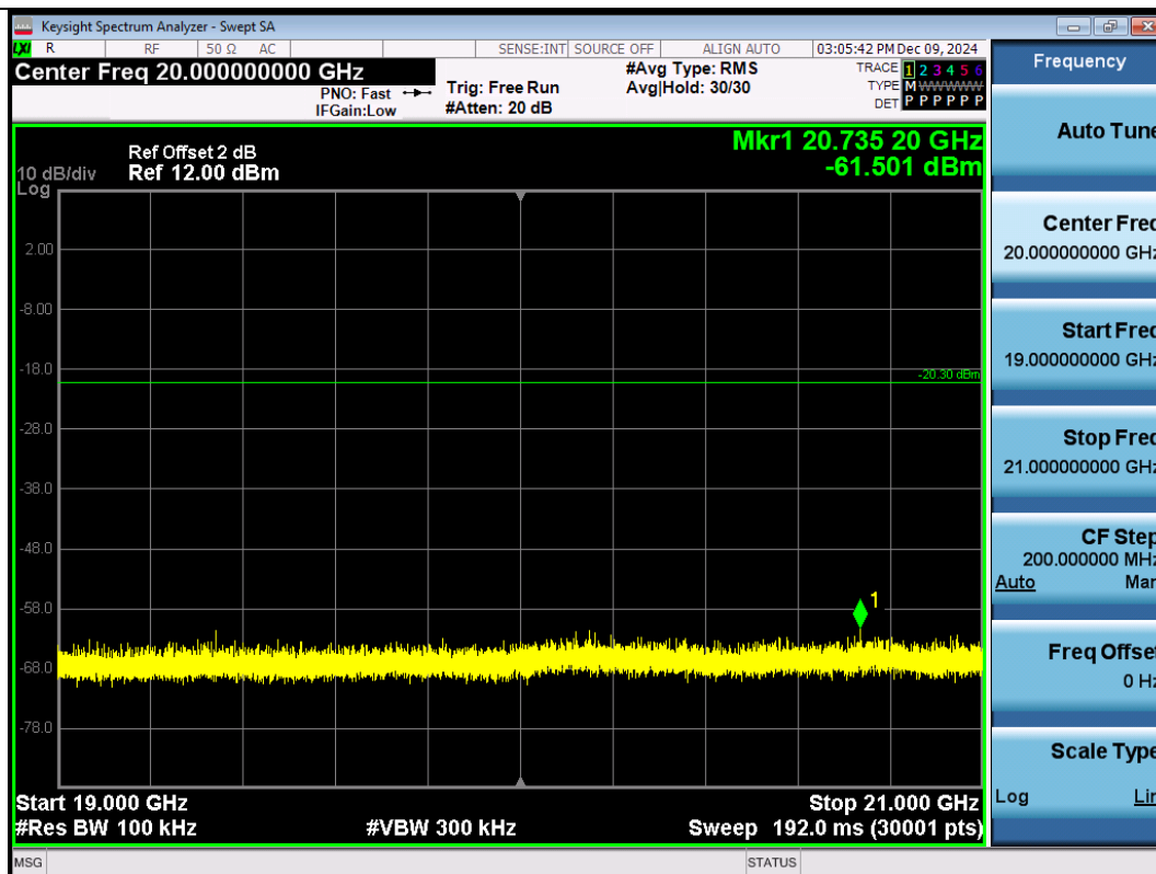
11B-Ant1-2412-19000-21000-PASS
