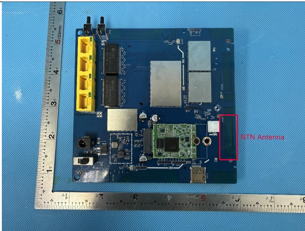
EUT Photo(9) WWAN NTN Antenna
