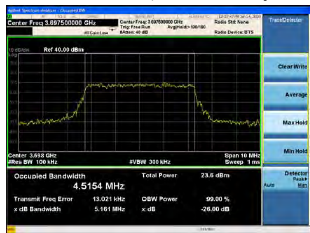
LTE Band 48 16QAM 5MHz CH-High
