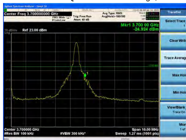
LTE Band 48 QPSK 10MHz CH-High, 1RB
