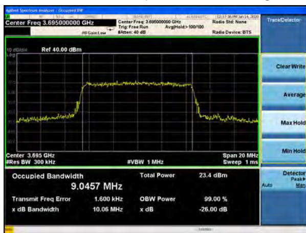
LTE Band 48 16QAM 10MHz CH-High
