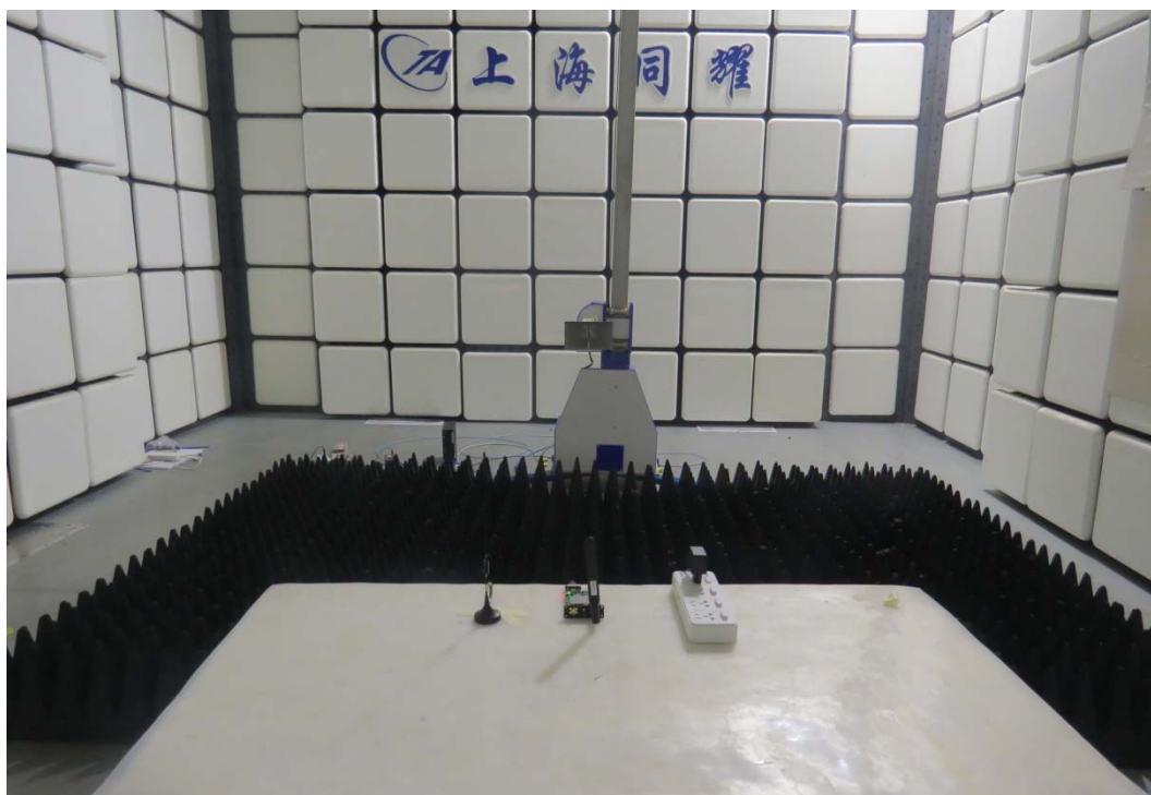
Picture 1 Radiated Emission Test Setup
