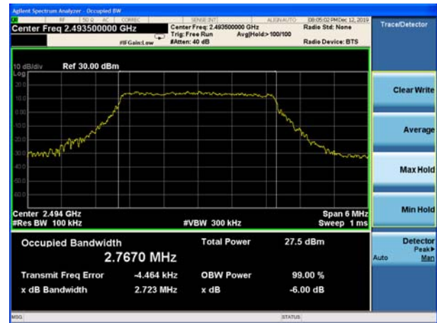
LTE Band 53 3MHz QPSK CH-High
