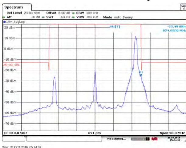
LTE Band 26 QPSK 10MHz CH-High 100%RB
