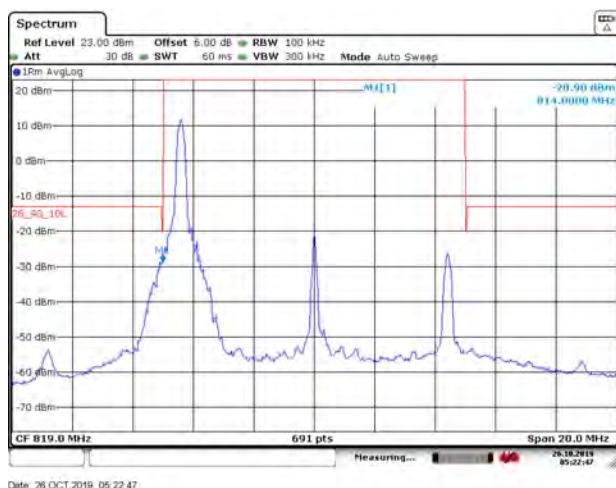
LTE Band 26 QPSK 10MHz CH-Low 100%RB
