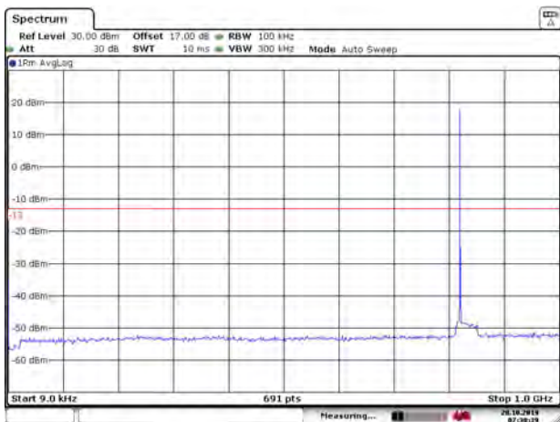
LTE Band 26 1.4MHz CH-Middle 9kHz~1GHz
