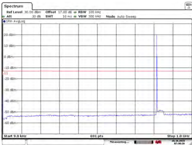
LTE Band 26 1.4MHz CH-Low 9kHz~1GHz
