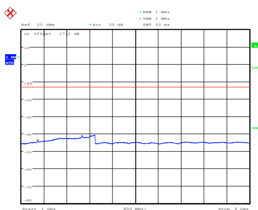
LTE Band 14 5MHz CH-Low 1GHz~9GHz
