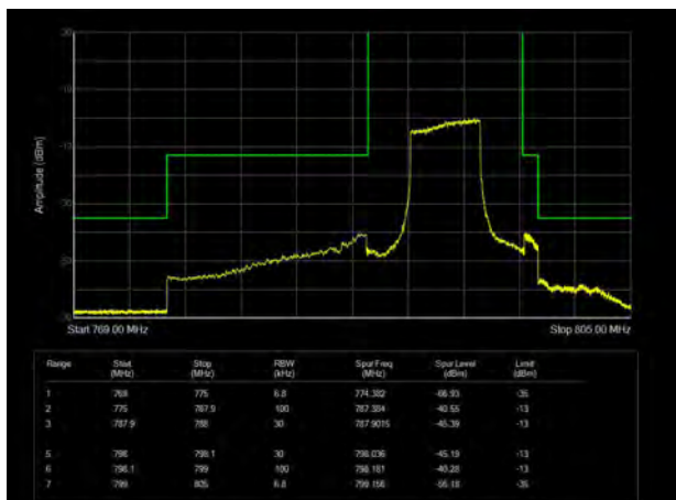
LTE Band 14 64QAM 10MHz 1 RB CH-23230
