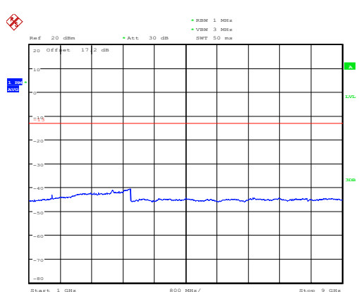
LTE Band 14 5MHz CH- Middle 1GHz~9GHz
