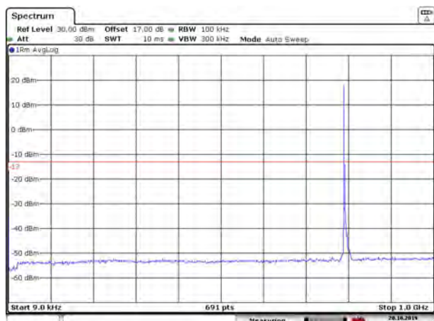
LTE Band 14 5MHz CH-Low 9kHz~1GHz
