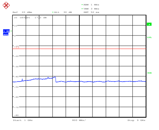
LTE Band 14 5MHz CH-High 1GHz~9GHz
