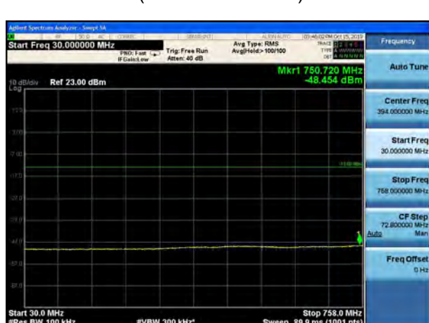
LTE Band 14 QPSK 5MHz 100%RB CH-High (30MHz ~758MHz)
