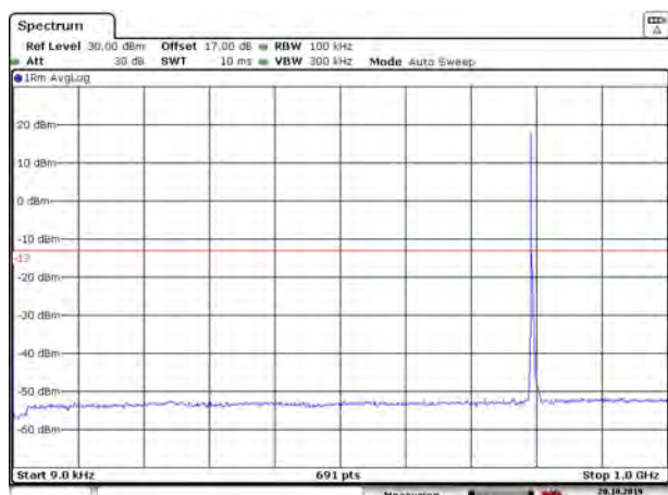
LTE Band 14 5MHz CH- Middle 9kHz~1GHz
