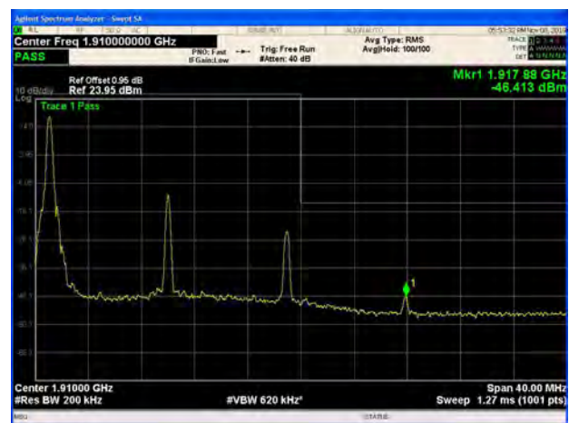
LTE Band 2 20MHz 64QAM 100%RB CH-High
