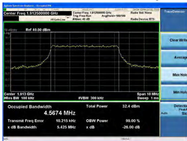
LTE Band 25 5MHz QPSK CH-High
