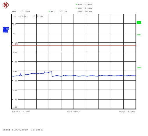
LTE Band 14 5MHz CH-High 1GHz~9GHz
