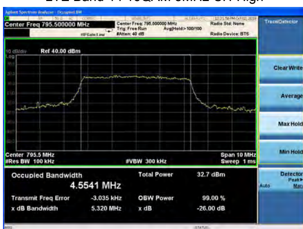
LTE Band 14 16QAM 5MHz CH-High
