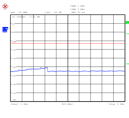
LTE Band 14 5MHz CH-Low 1GHz~9GHz
