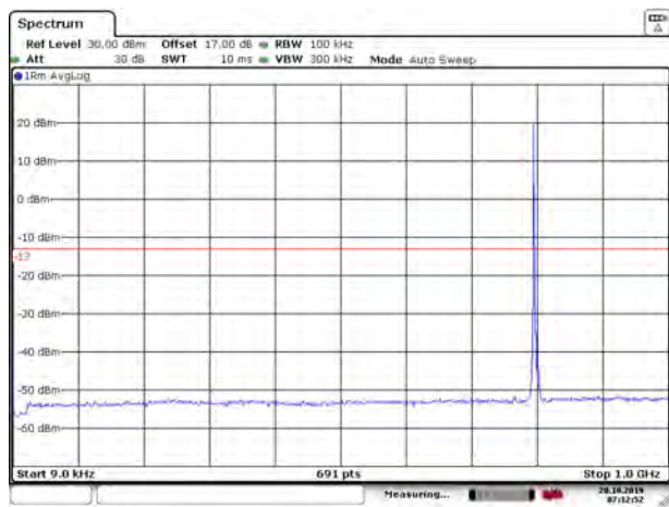
LTE Band 14 5MHz CH-High 9kHz~1GHz
