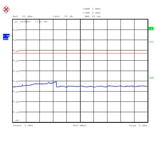
LTE Band 14 5MHz CH- Middle 1GHz~9GHz
