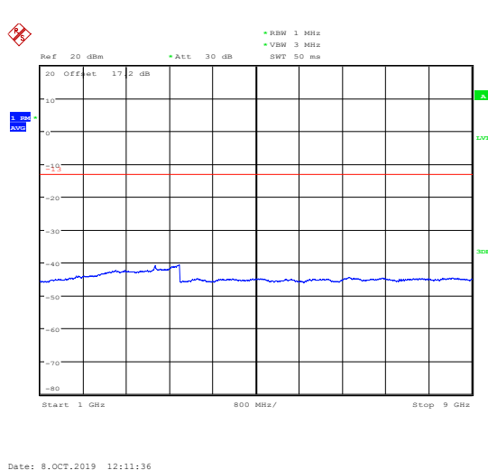
LTE Band 5 1.4MHz CH-Middle 1GHz~9GHz
