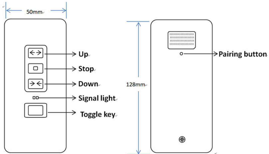
S802G02 Front view
