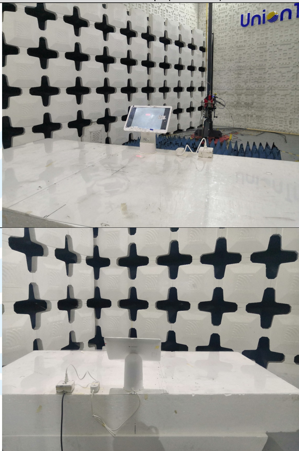
Radiated emission Test Setup-2 (Above 1 GHz) - Mode 3
