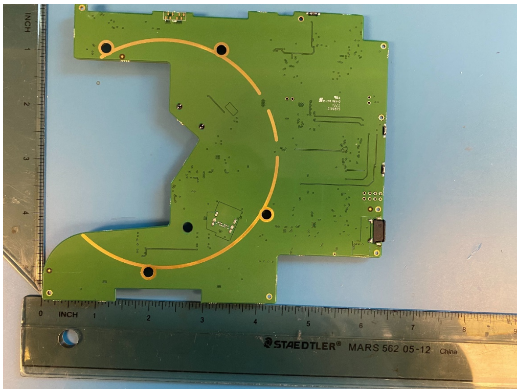
Figure 6: Backside of Control board
