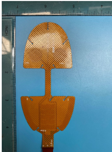
Figure 13: Capsense Flex
