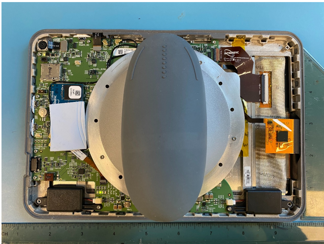
Figure 14: Tablet without backcover
