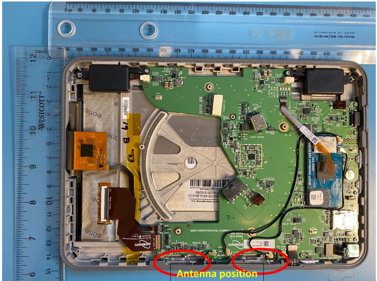
Figure 1: Back cover and table handle removed
