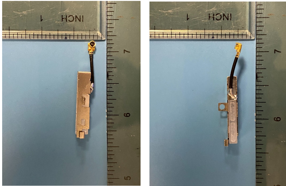
Figure 11: PIFA antennas 2.4GHz/5.0 GHz Wifi and Bluetooth
