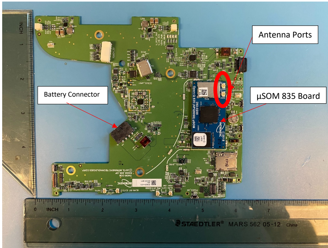
Figure 5: Front view of Control board
