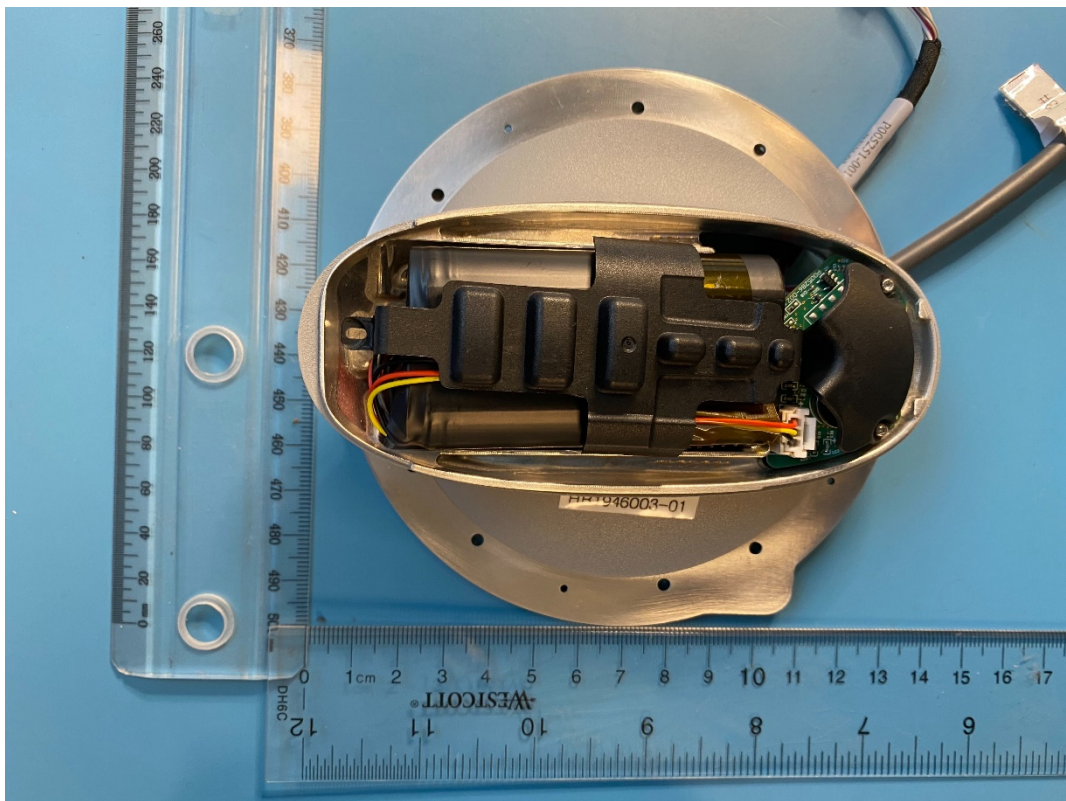
Figure 2: Battery handle with rubber cap removed
