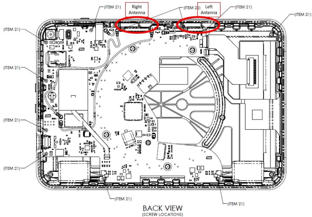
FIGURE 1 : REAR VIEW OF THE DISSASSEMBLED THOR TABLET
