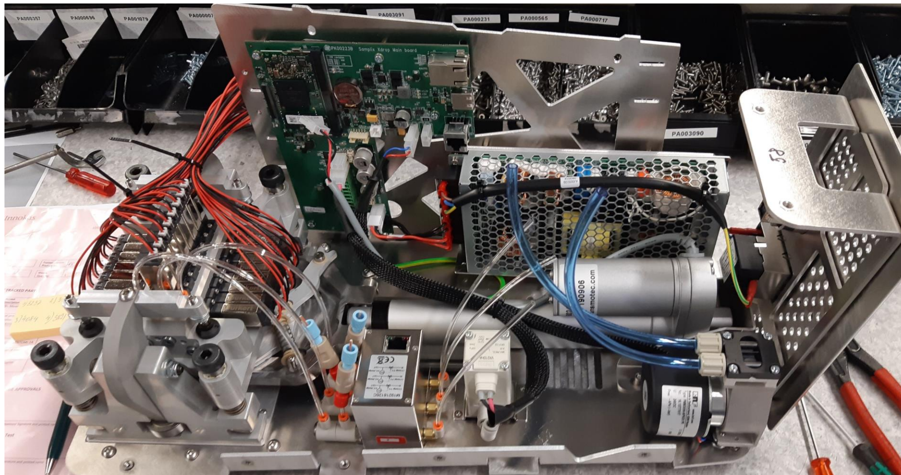
Figure 1 Inside Xdrop (side panel removed)
