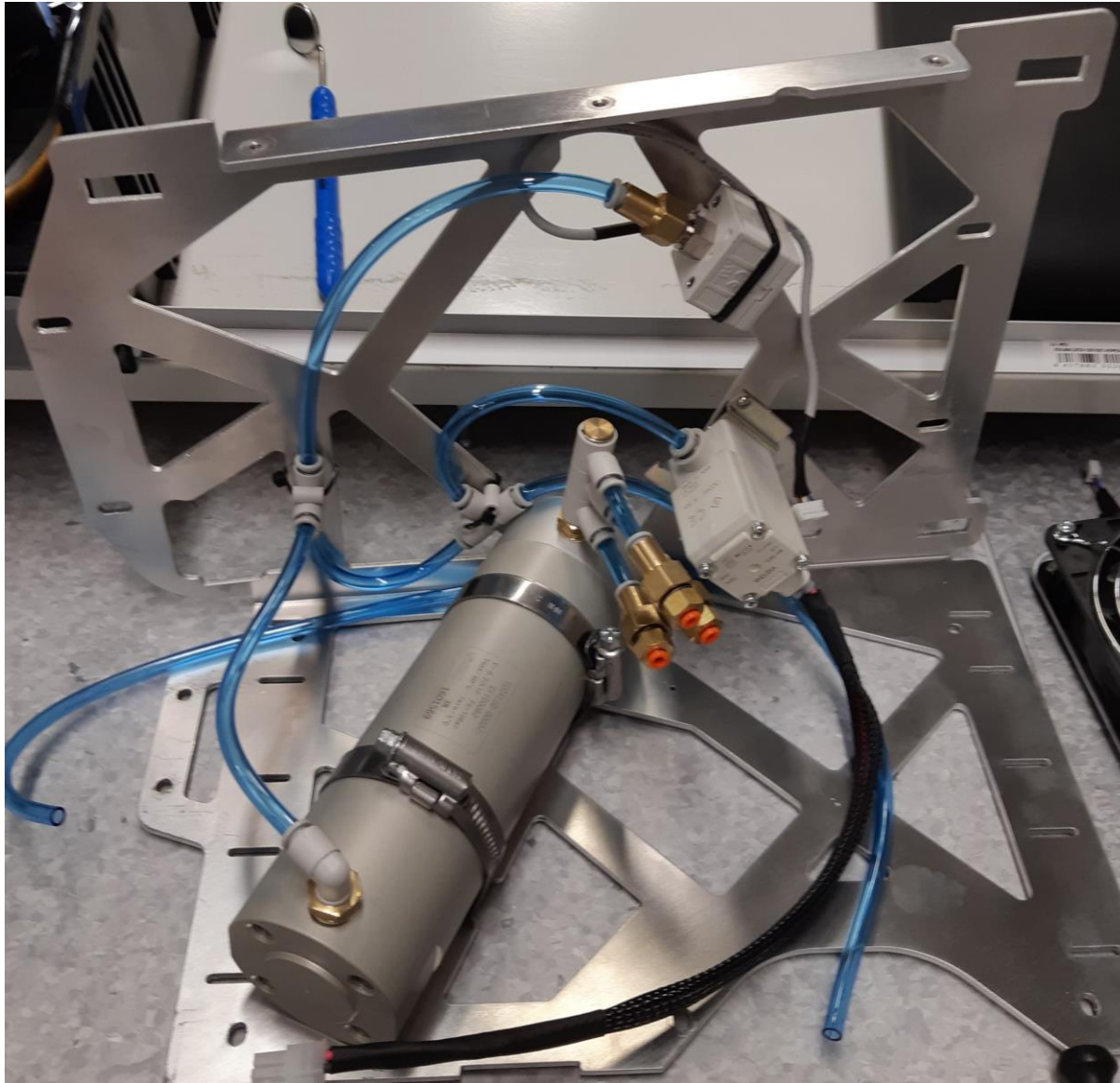
Figure 4 - Frame and air vessel
