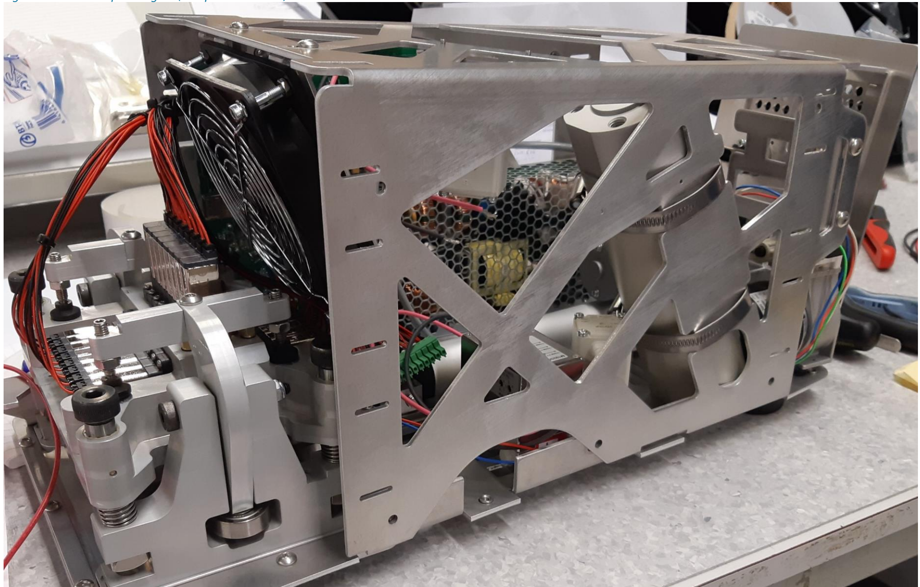
Figur 1 - Inside Xdrop – image 2 (side panel attached)
