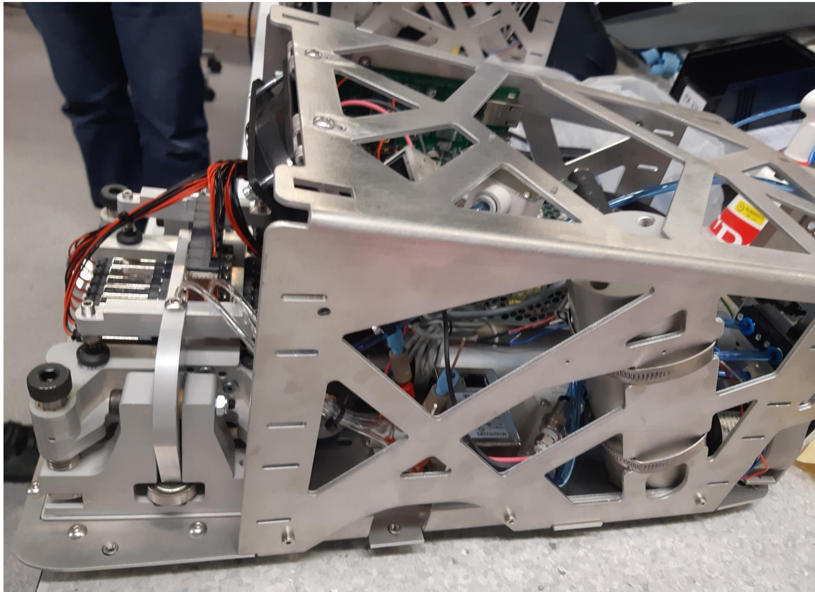
Figure 2 - Inside Xdrop (side panel attached)
