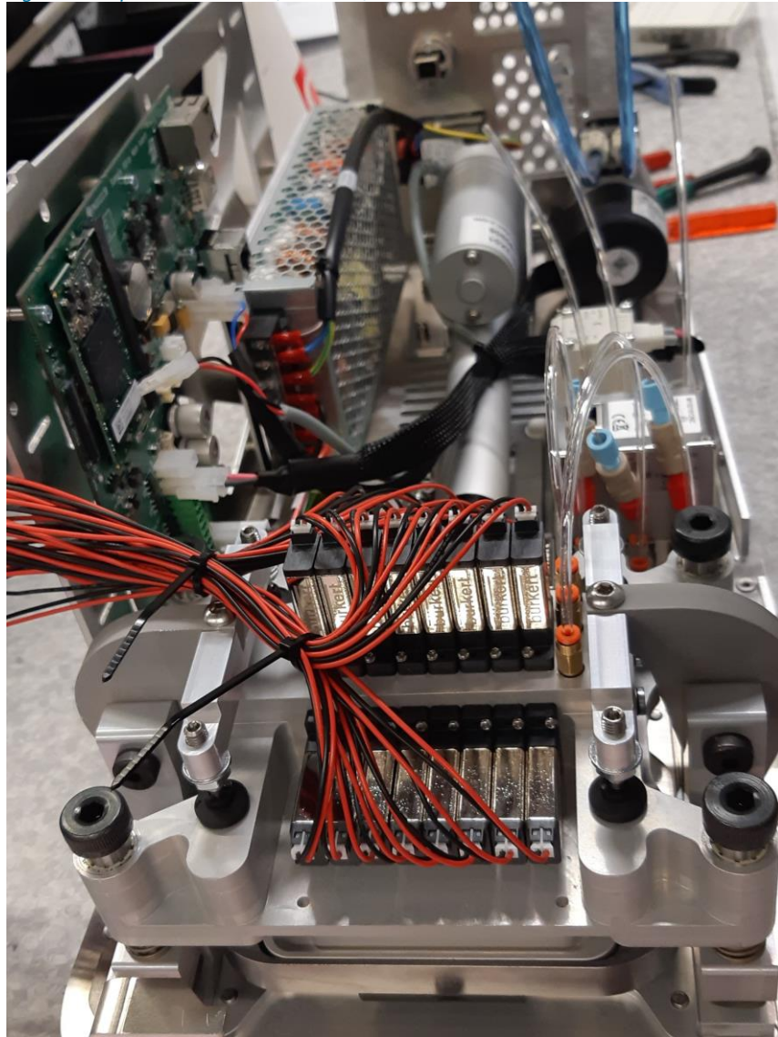
Figure 3 - Open instrument (from the front)
