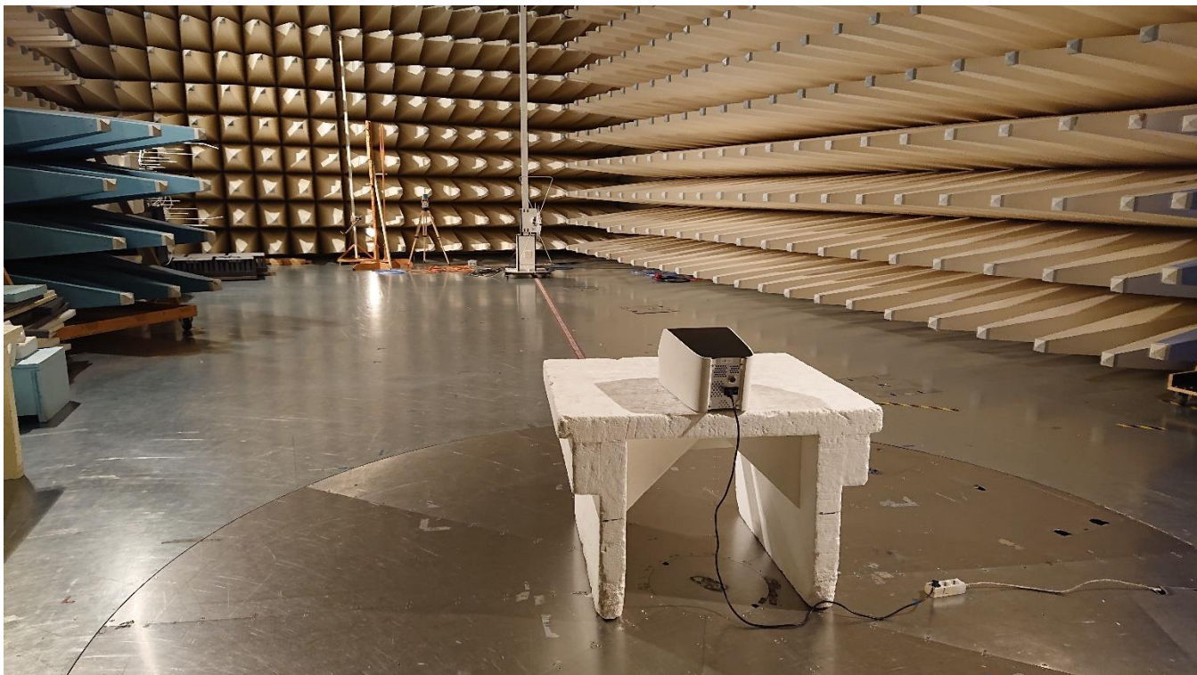
Photograph 5. Radiated Emissions 30 – 1000 MHz
