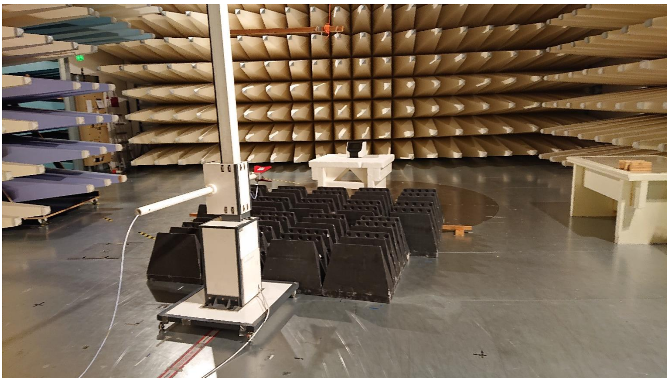
Photograph 6. Radiated Emissions 1 – 5 GHz
